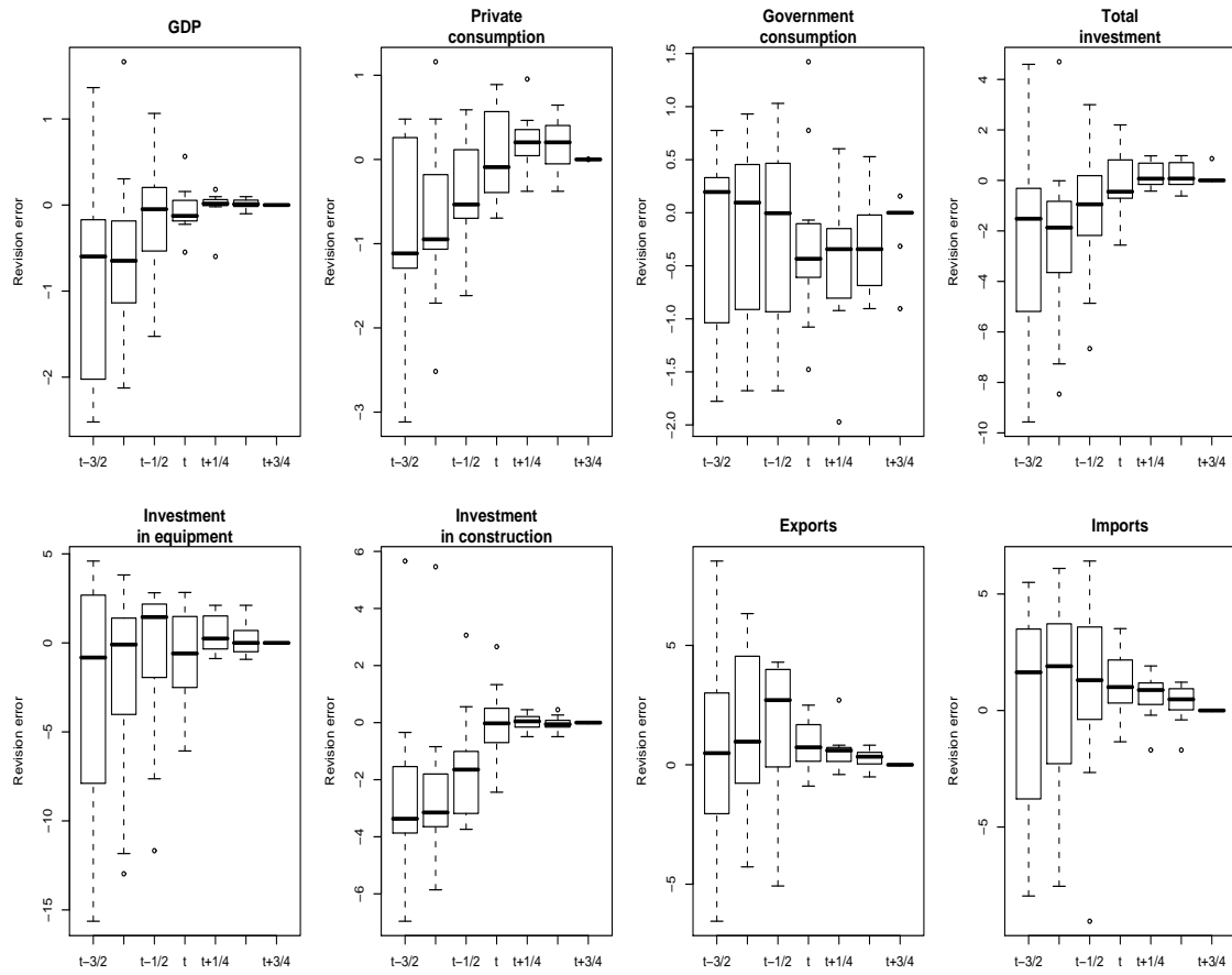
Figure 5: Real variables: Distribution of the forecast/revision errors
