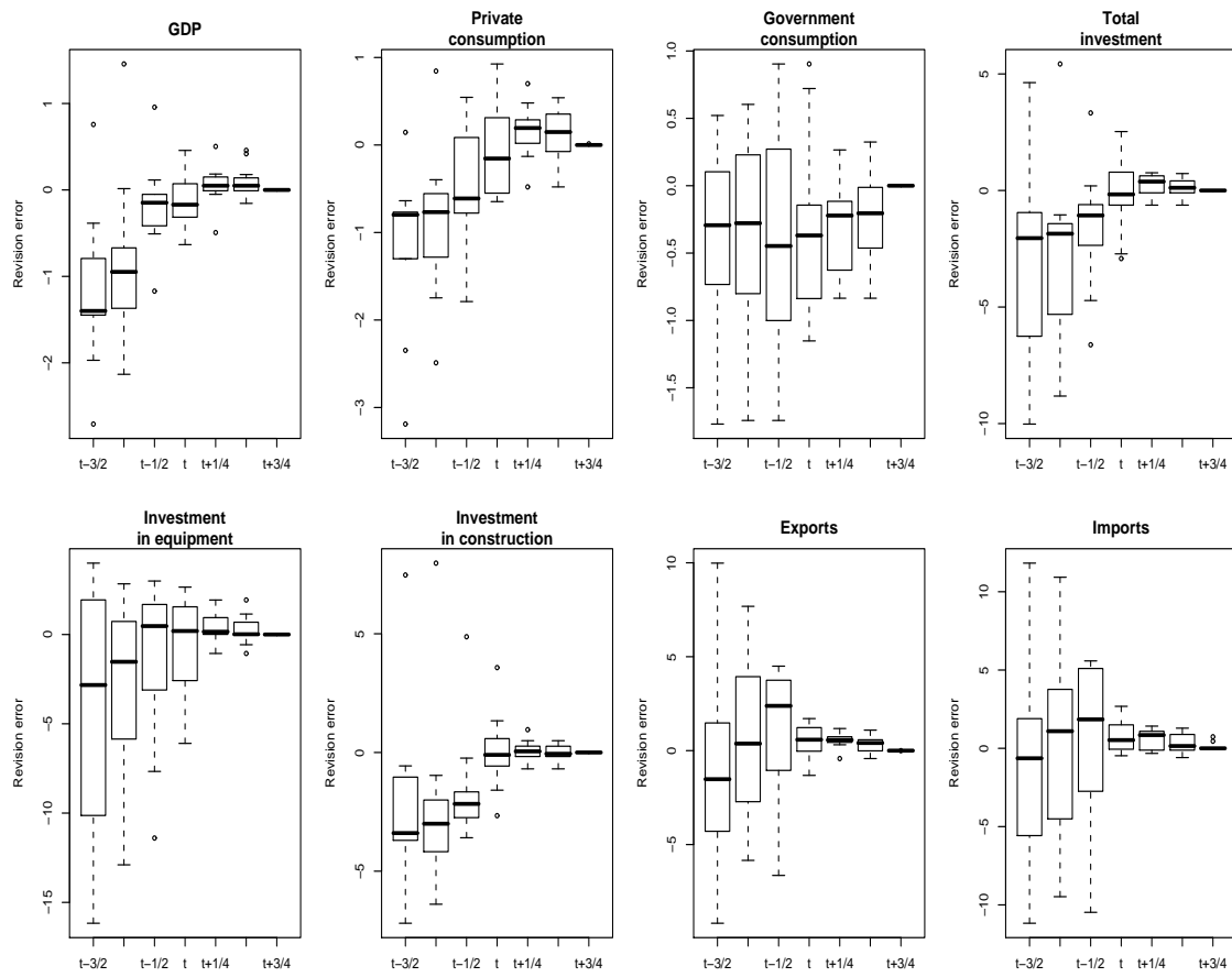
Figure 4: Nominal variables: Distribution of the forecast/revision errors
