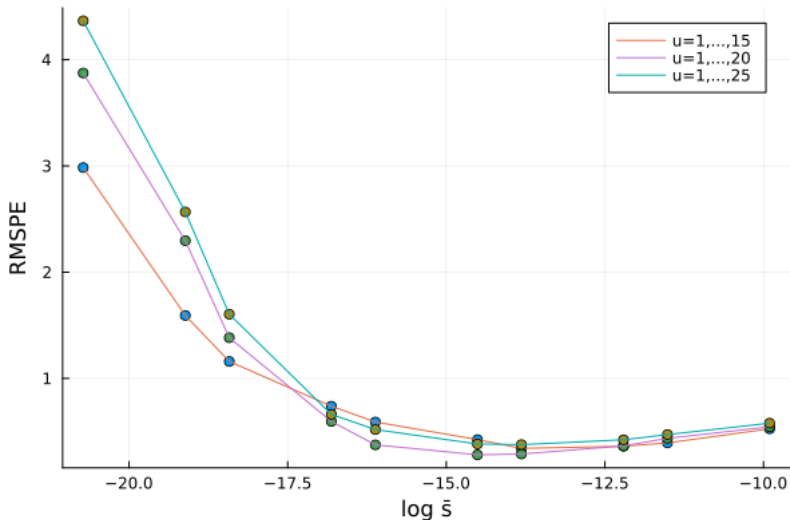
Figure 1: RMSPE for different levels of \bar{s}
