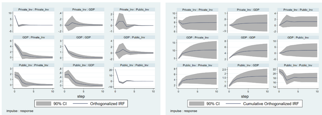
Figure 4: IRFs from PVAR with public investment in European regions
