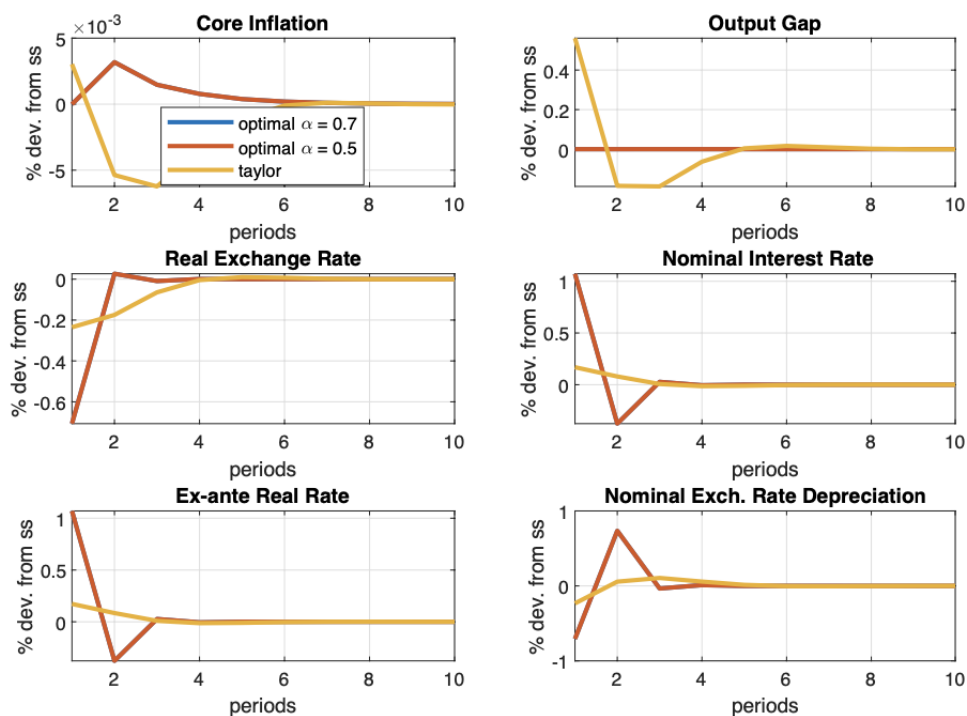
Figure 2: Impulse Response Functions: Demand Shock.
