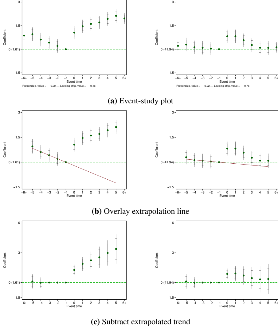
Figure 8: Illustration of approach based on extrapolating confound from pre-event periods. Each column of plots corresponds to a different possible dataset. Panel (a) shows the event-study plot. Panel (b) extrapolates a linear event-time trend from the three immediate pre-event periods, as in Dobkin et al. (2018). It then overlays the event-time coefficients for the trajectory of the dependent variable and the extrapolated linear trend. In Panel (c), the estimated effect of the policy is the deviation of the event-time coefficients of the dependent variable from the extrapolated linear trend. Note that the y-axis in Panel (c) differs from that in (a) and (b).
