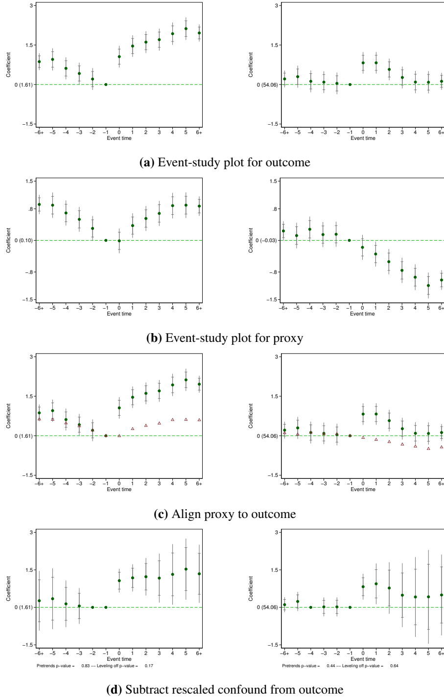
Figure 9: Illustration of use of a proxy to adjust for confound. Each column of plots corresponds to a different possible dataset. Panel (a) shows the event-study plot for the outcome. Panel (b) shows the event-study plot for the proxy. Panel (c) overlays the point estimates from Panel (b) on the plot from Panel (a), aligning the coefficients at two event times. Panel (d) adjusts for the confound using the 2SLS estimator proposed in Freyaldenhoven et al. (2019).
