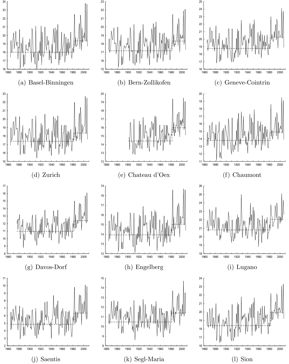
Figure 1: Observed annual maximum temperature (solid line) and the estimated location parameter of the fitted GEV distribution (dashed line)
