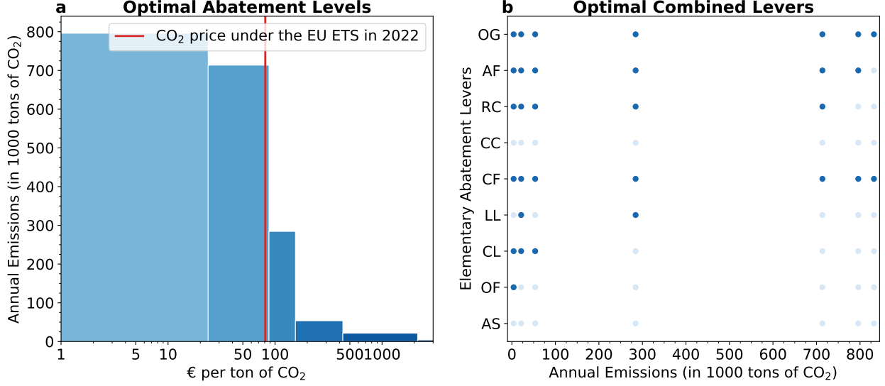
Supplemental Figure 2. Optimal abatement for Portland Cement. This figure shows (a) the optimal abatement at different CO 2 prices and (b) the optimal combined levers for increased cement output. Abbreviations are OG (Optimized Grinding), AF (Alternative Fuels), RC (Recycled Concrete), CC (Calcined Clays), LL (LEILAC), CL (Calcium Looping), OF (Oxyfuel), and AS (Amine Scrubbing).
