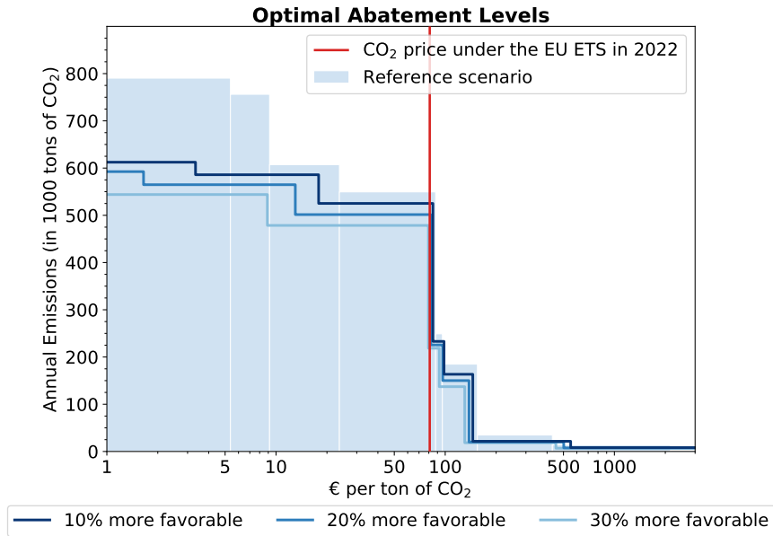
Supplemental Figure 10. Optimal abatement for Portland Cement. This figure shows the optimal abatement at different CO 2 prices for more favorable cost and abatement parameters. The optimal combined levers underlying the abatement levels are provided in the Supplemental Data.
