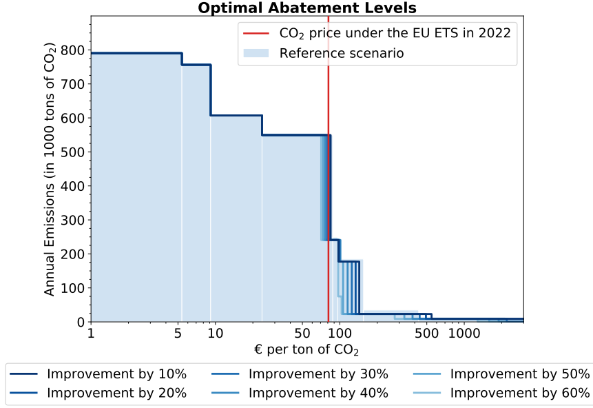
Supplemental Figure 8. Optimal abatement for Portland Cement. This figure shows the optimal abatement at different CO 2 prices assuming improvements in carbon capture technologies. The optimal combined levers underlying the abatement levels are provided in the Supplemental Data.
