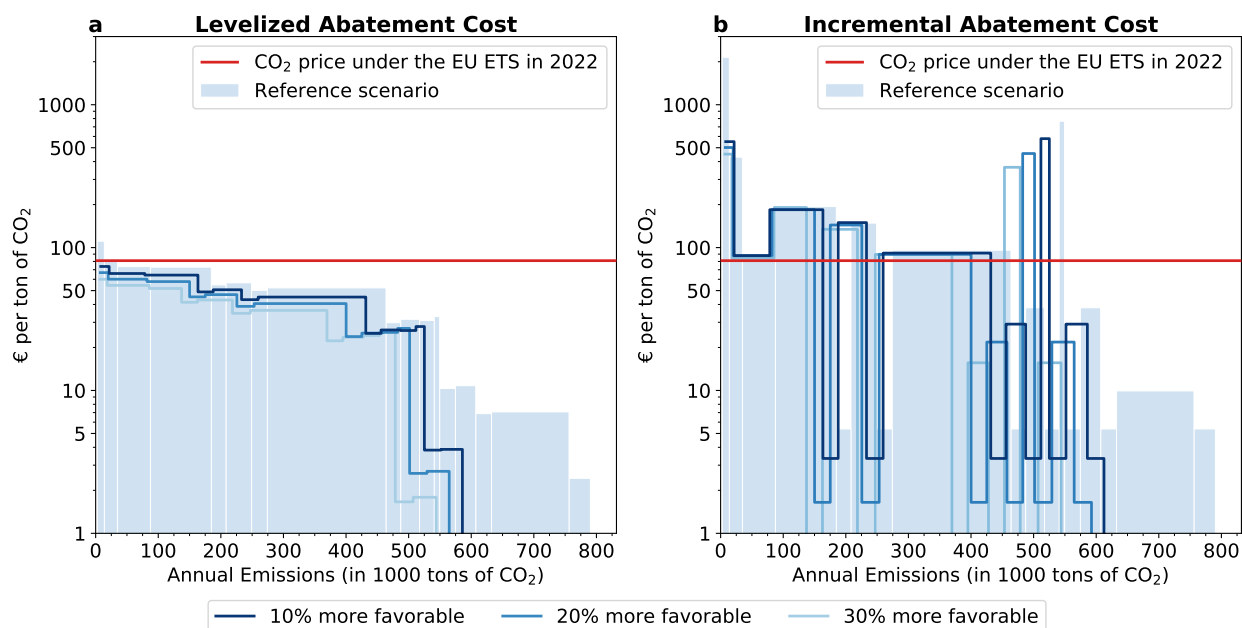
Supplemental Figure 9. Abatement cost curves for Portland cement. This figure shows the (a) levelized abatement cost and (b) incremental abatement cost for the cost-efficient emission thresholds for more favorable cost and abatement parameters.
