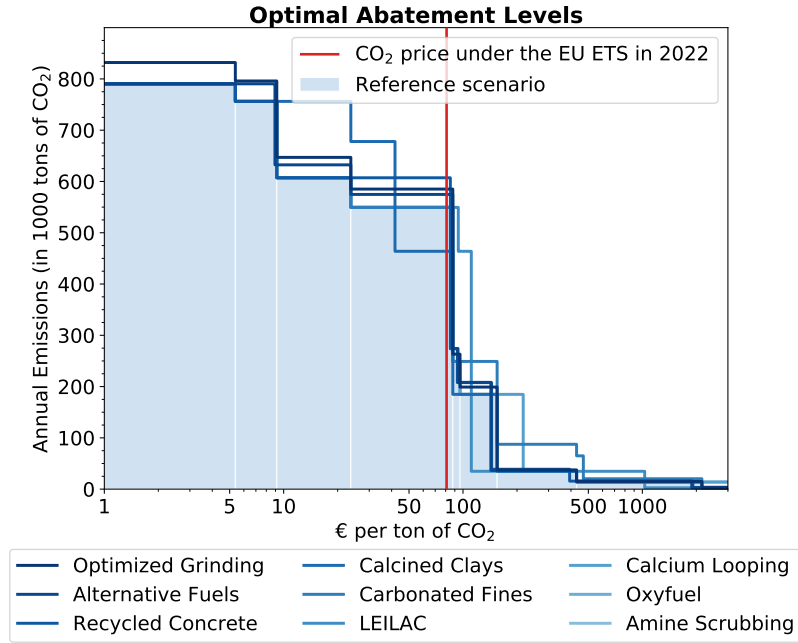
Supplemental Figure 4. Optimal abatement for Portland Cement. This figure shows the optimal abatement levels at different CO 2 prices, assuming one elementary lever is unavailable. The optimal combined levers underlying the abatement levels are provided in the Supplemental Data.
