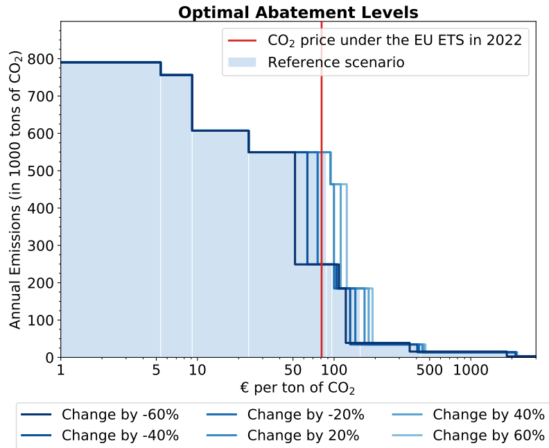
Supplemental Figure 6. Optimal abatement for Portland Cement. This figure shows the optimal abatement at different CO 2 prices for alternative changes in the costs of transporting and storing captured CO 2 . The optimal combined levers underlying the abatement levels are provided in the Supplemental Data.
