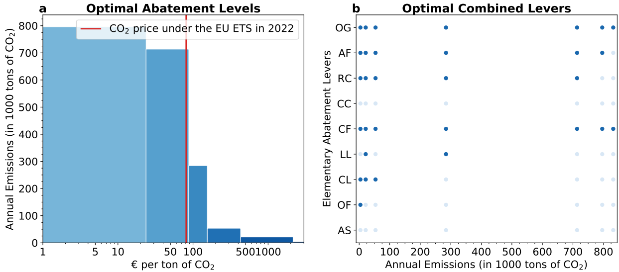
Supplemental Figure 2. Optimal abatement for Portland Cement. This figure shows (a) the optimal abatement at different CO 2 prices and (b) the optimal combined levers for increased cement output. Abbreviations are OG (Optimized Grinding), AF (Alternative Fuels), RC (Recycled Concrete), CC (Calcined Clays), LL (LEILAC), CL (Calcium Looping), OF (Oxyfuel), and AS (Amine Scrubbing).
