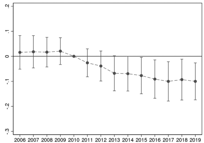
Fig. 3. Event studies – expenses.
