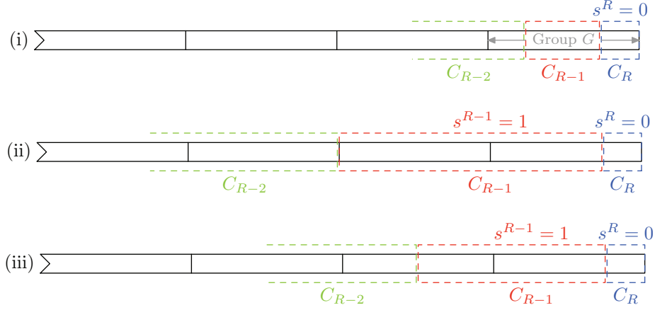
Figure A.2: The last class C_R
