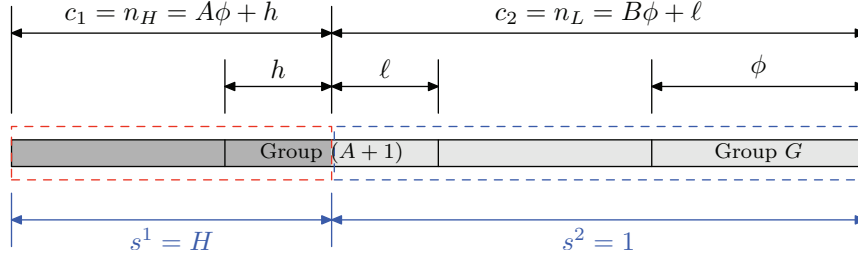
Figure 3.2: The distribution of players in a FEE
