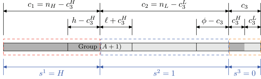
Figure 3.4: The distribution of players in a NEE
