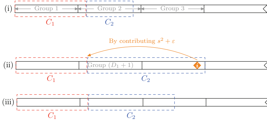
Figure A.1: There is at least one High in C_1
