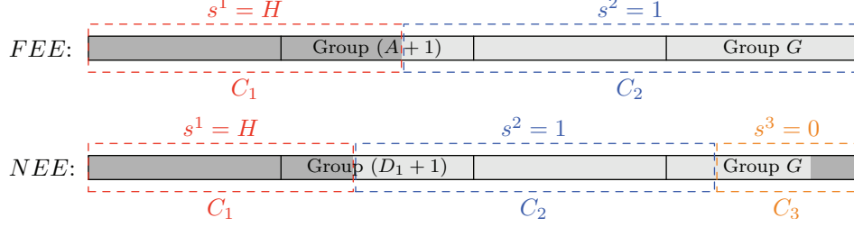
Figure 3.1: The two equilibrium configurations with positive contributions (light grey sections are Lows, dark grey sections are Highs)
