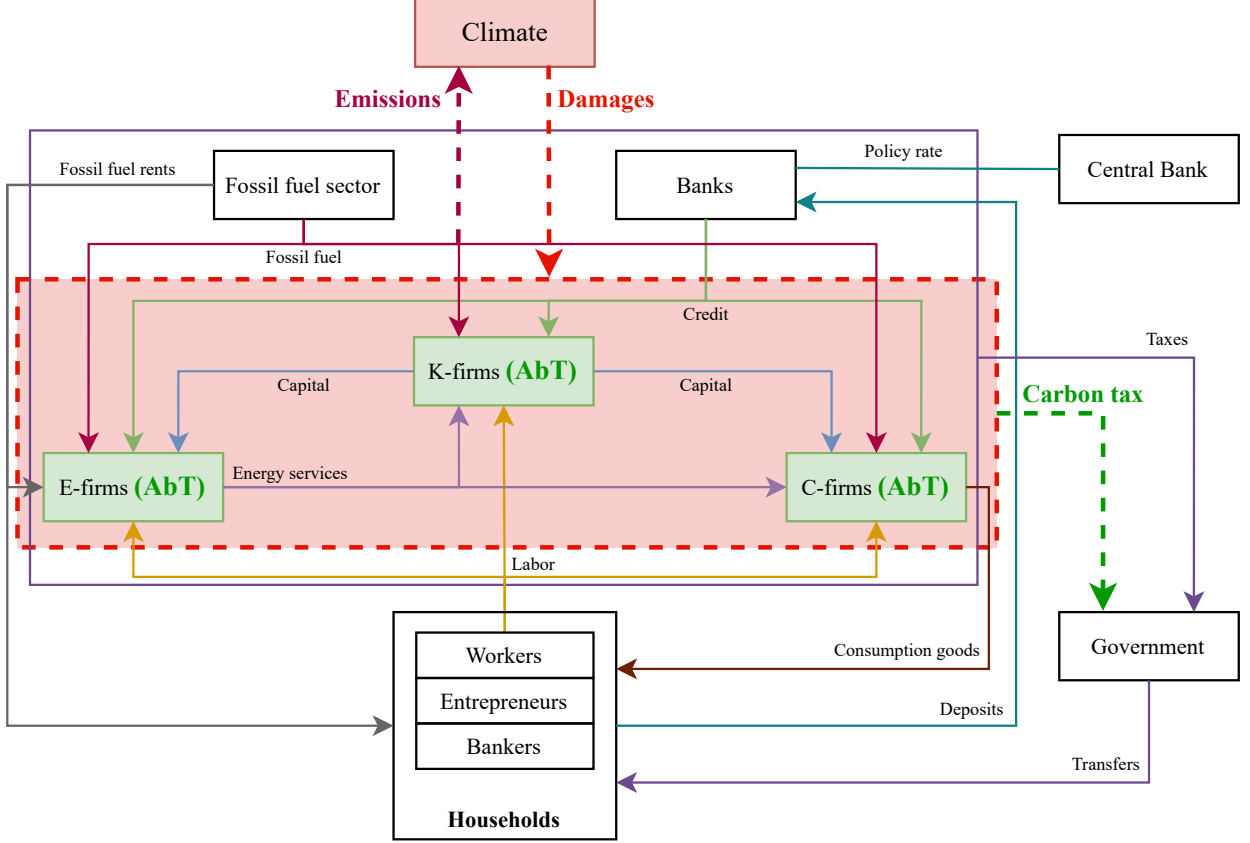
Figure 1: The MATRIX model and climate extensions (dashed lines and shaded areas)
