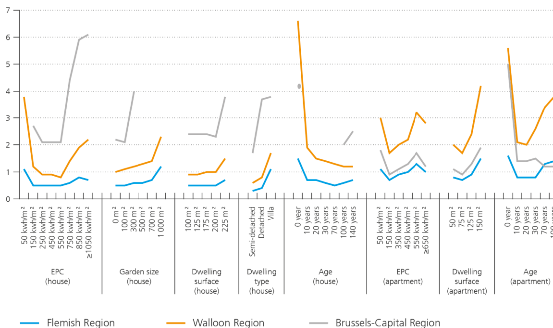
Chart 17 - Standard error for a selection of estimated (untransformed) coefficients in 2021 (in %)
