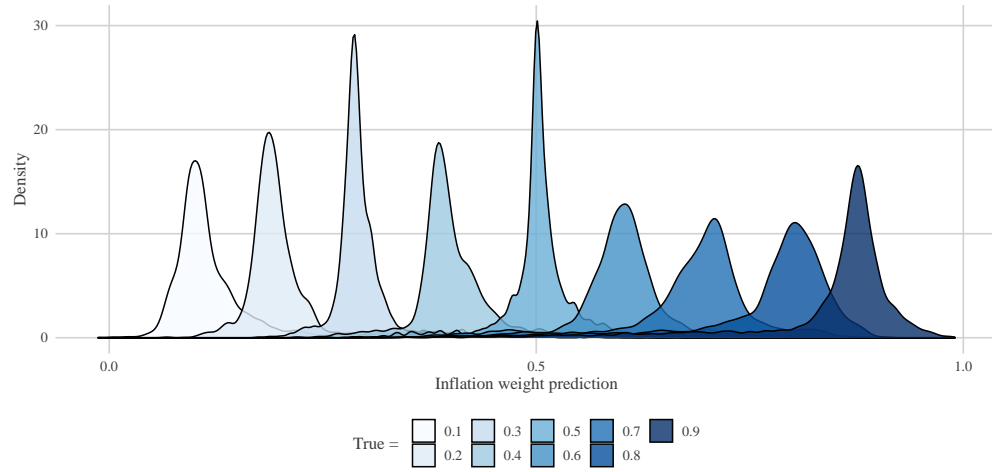
Figure A1.1 : Density Forecasts - Out-of-Sample Predictions.
