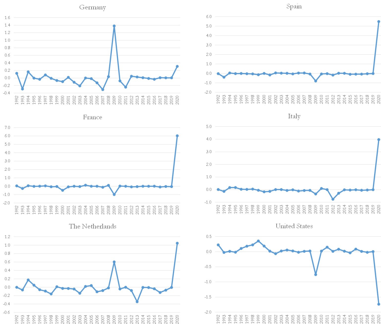
Figure 1: Influential observations: Output of a systematic DF-Beta analysis
