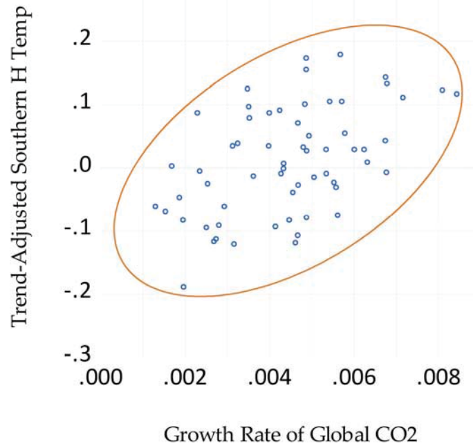
Figure (13a) Chi-Squared 95% Confidence Ellipse
