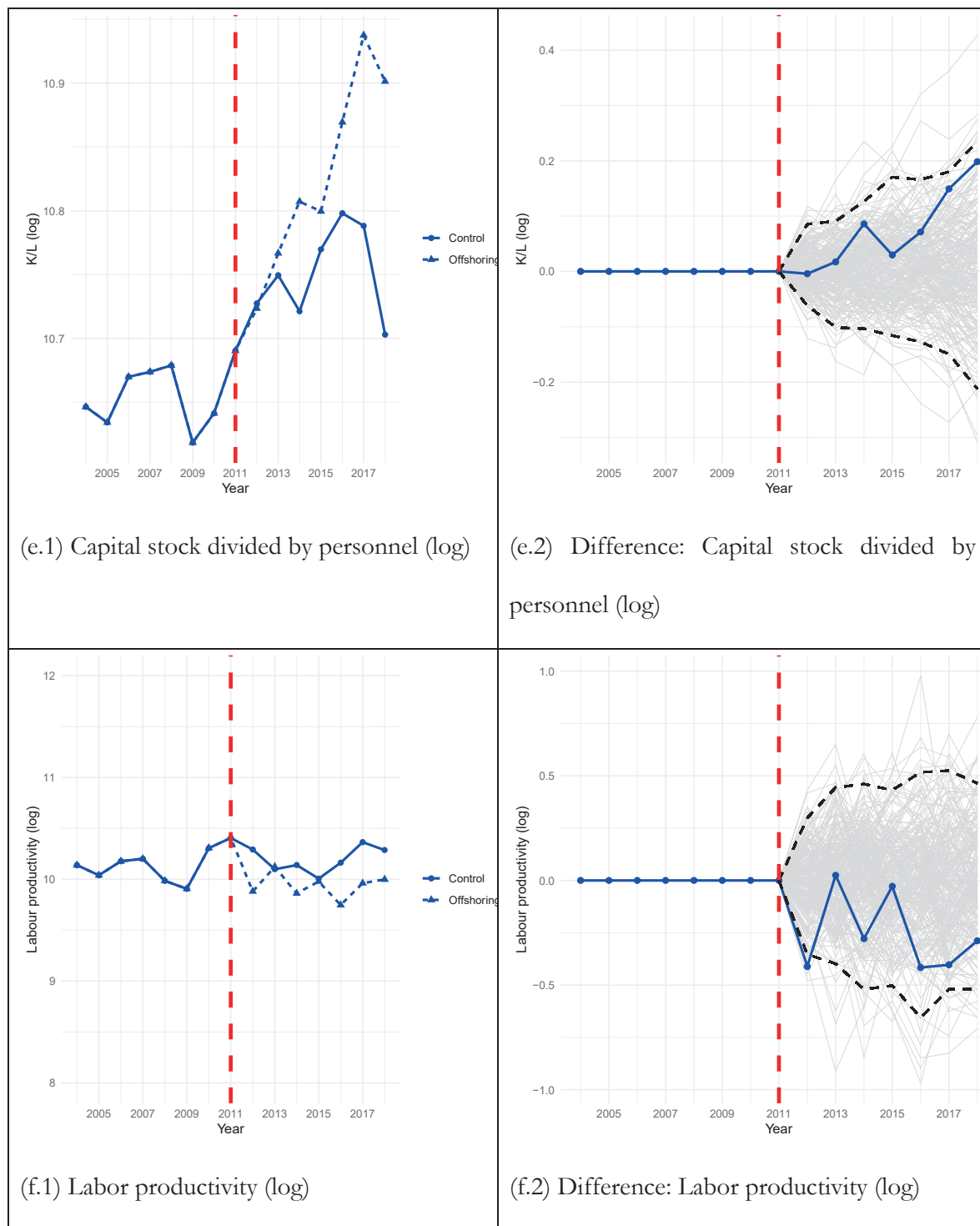
Figure 2. A comparison between the offshoring firms and the synthetic control in levels (a.1–f.1) and differences between the two (a.2–f.2). The red vertical line corresponds to the year 2011, which is the treatment date. In a.1–f.1, the solid line is the synthetic control and the dashed line is the
