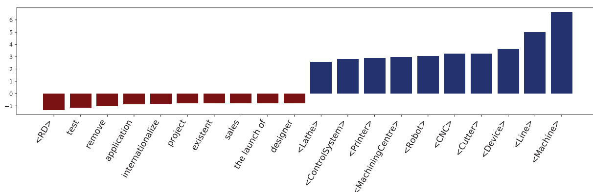
Figure E1: Predictive Features for Text Categories: Technology.
