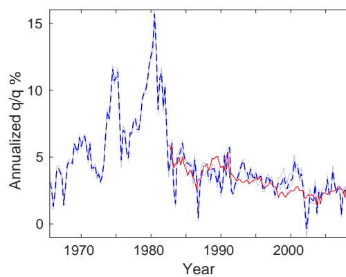
(e) VAR(1)
