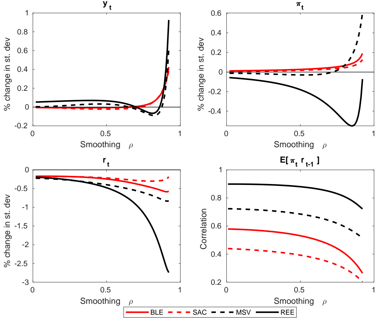
Figure 5: Standard deviations (y-axis) as a function of interest rate smoothing \rho (x-axis). Solid lines correspond to equilibrium models (BLE and REE), while dashed lines are learning models (SAC- and pseudo MSV-learning). Red lines correspond to a PLM with AR(1) rule (BLE and SAC), whereas black lines correspond to REE-consistent rules (REE and pseudo MSV-learning).
