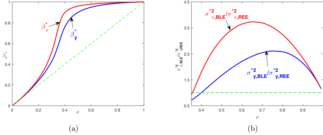
Figure 2: BLE (\beta_y^*, \beta_\pi^*) as a function of the persistence \rho of the exogenous shocks. (a) \beta_i^*(i = y, \pi) with respect to \rho ; (b) the ratio of variances (\sigma_{y,BLE}^{*2}/\sigma_{y,REE}^{*2}, \sigma_{\pi,BLE}^{*2}/\sigma_{\pi,REE}^{*2}) of the BLE (\beta_y^*, \beta_\pi^*) w.r.t. the REE. Parameters are: \lambda = 0.99, \varphi = 1, \gamma = 0.04, \phi_\pi = 1.5, \phi_y = 0.5, \frac{\sigma_\pi}{\sigma_y} = 0.5 .
