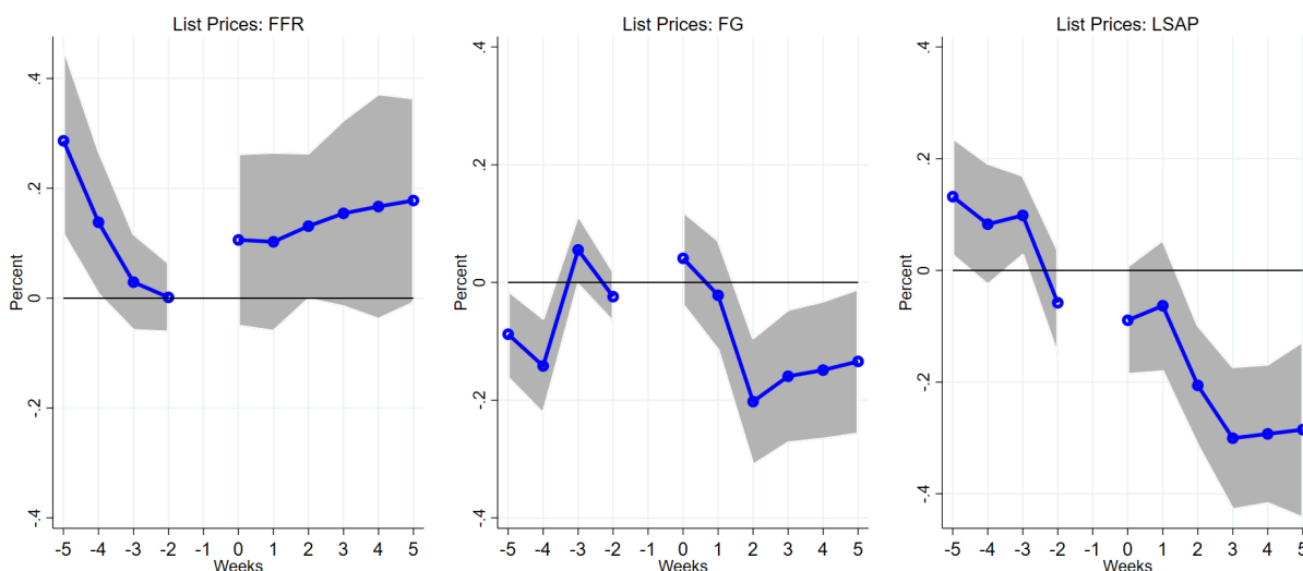
Figure B.1. Responses of Housing List Prices to Contractionary Monetary Policy Surprises
