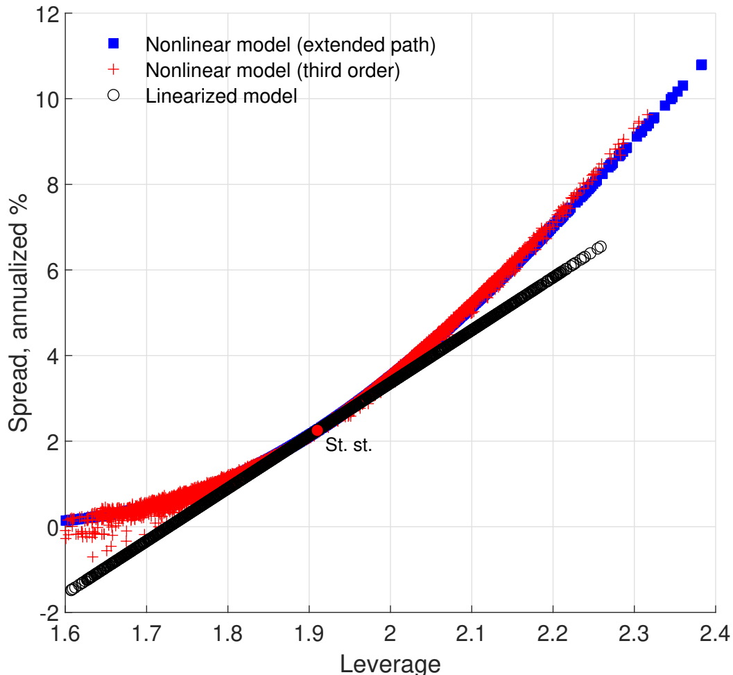
Figure 2: Leverage-spread schedule
