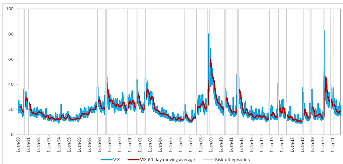
Figure 1: Risk-off Episodes, 1990–2021
