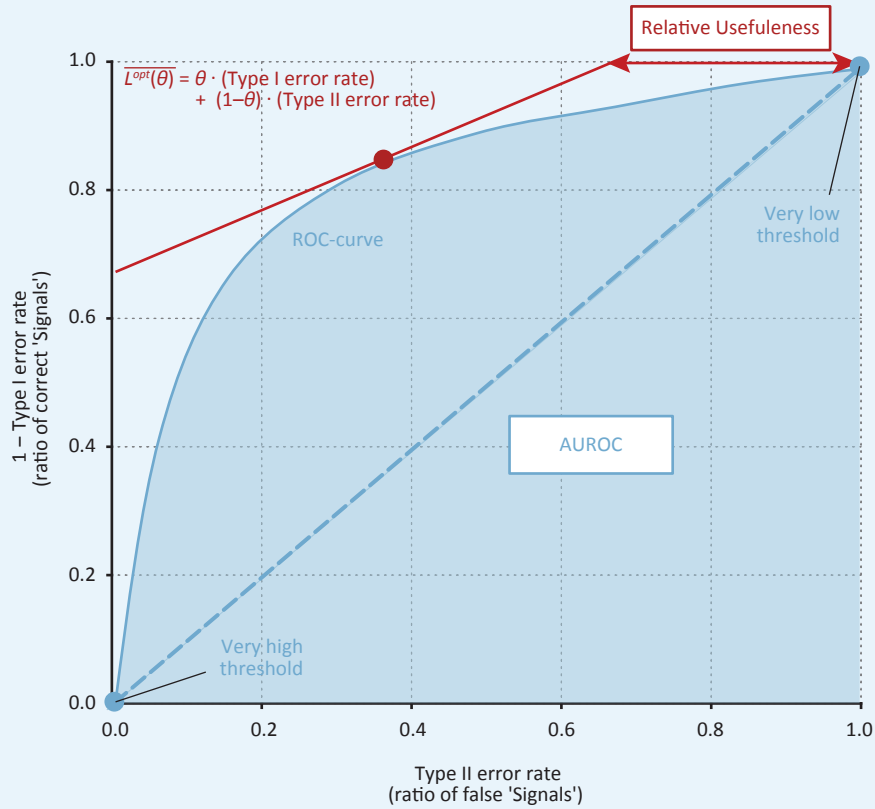
Figure 12 Relationship between Type I errors, Type II errors, AUROC criterion, and RU criterion
