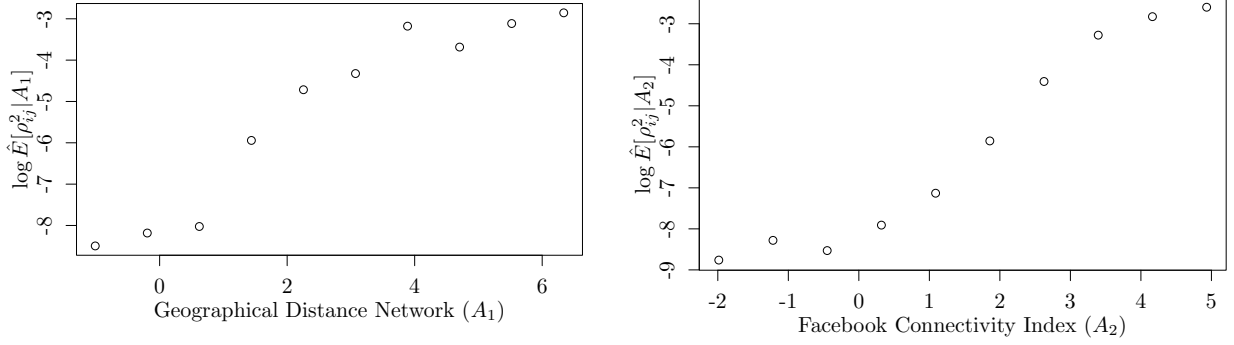
Figure A.5: Assessing the linear relation between \log \mathbb{E}[\hat{\rho}_{jk}^2 | A] and the network matrices, where \hat{\rho}_{jk} is the GLASSO estimate. The points represent the log-mean values of \hat{\rho}_{jk}^2 within 10 equispaced bins defined for each network.
