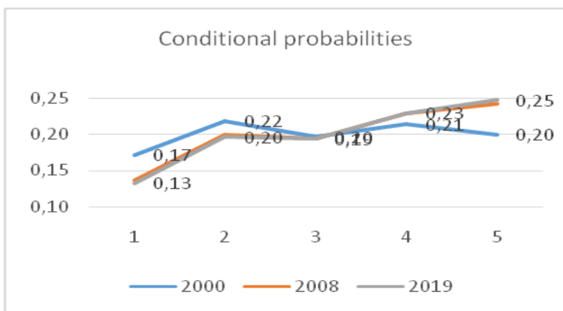
Fig.11. Conditional probabilities for being in quintiles 1 to 5, in 2000, 2008 and 2019.
