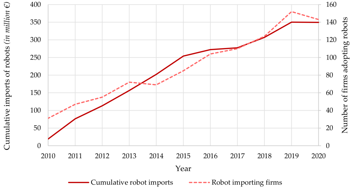
FIGURE 1 – CUMULATIVE ROBOT ADOPTION
