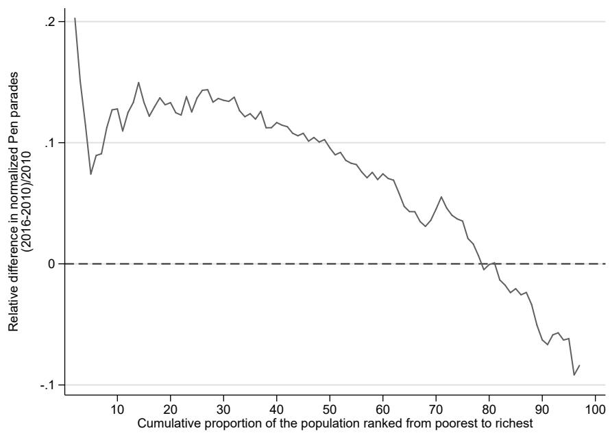
(b) Growth Incidence Curve
