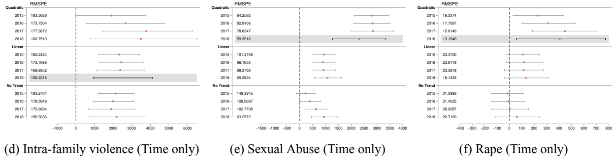
Figure 6: Projected Under-reporting under Various Counterfactual Assumptions
