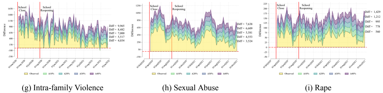
Figure 5: Reporting, Projected Reporting, and Under-reporting Under Various Counterfactual Assumptions
