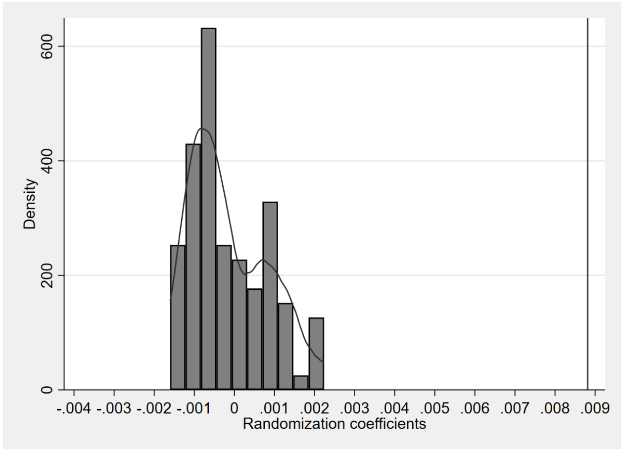
Figure 7: Randomization Test
