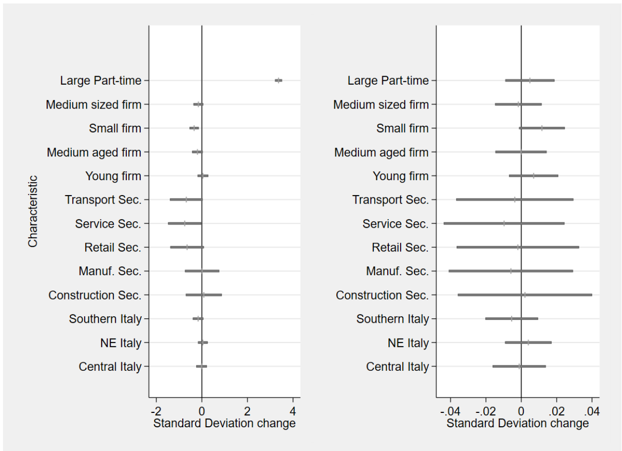
Figure 3: Balance Test
