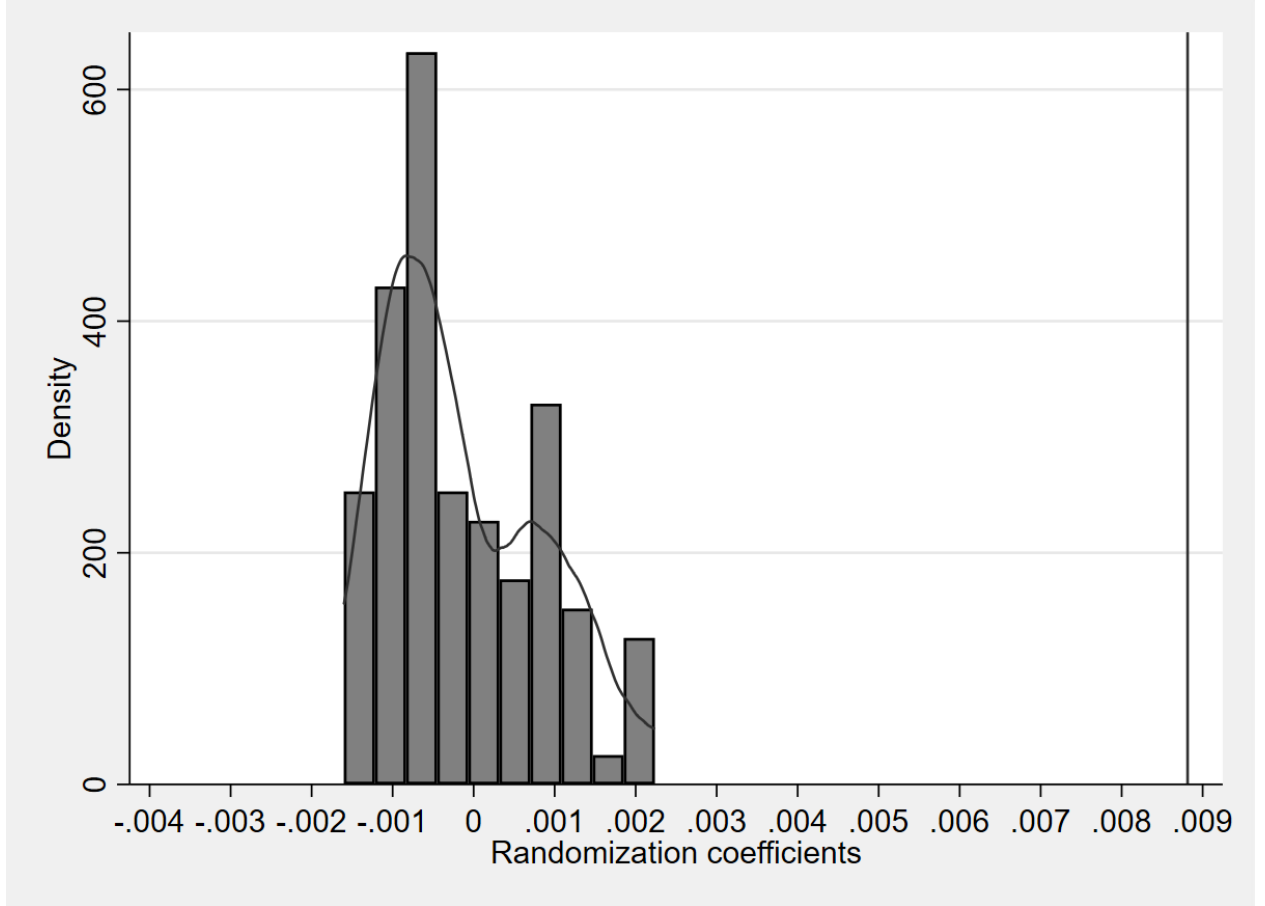
Figure 7: Randomization Test
