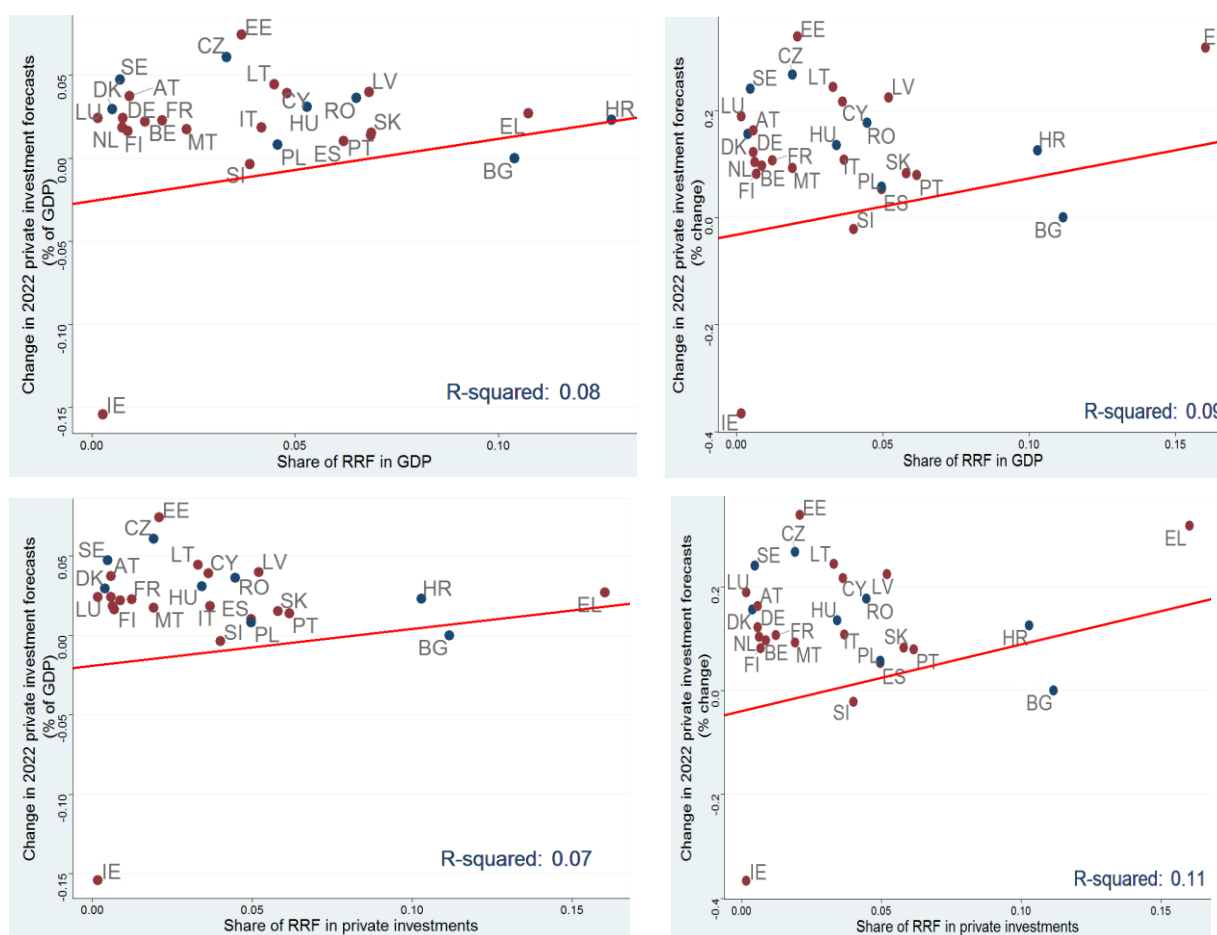
Figure 8: Graphical outputs of the four regression models for private investments
