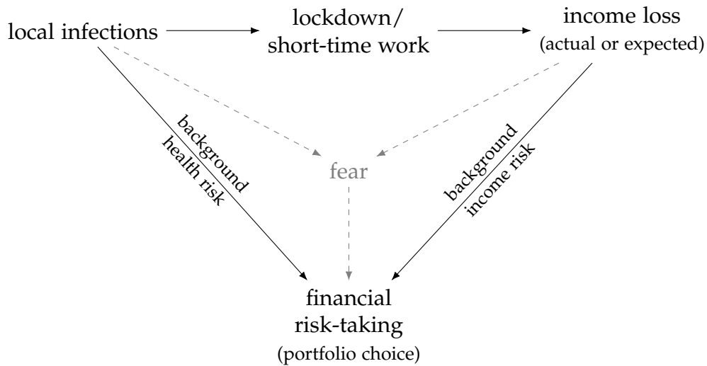
Figure A1: Conceptual Causal Diagram.
