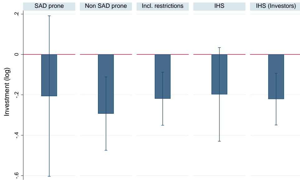
Figure 5: Robustness checks.
