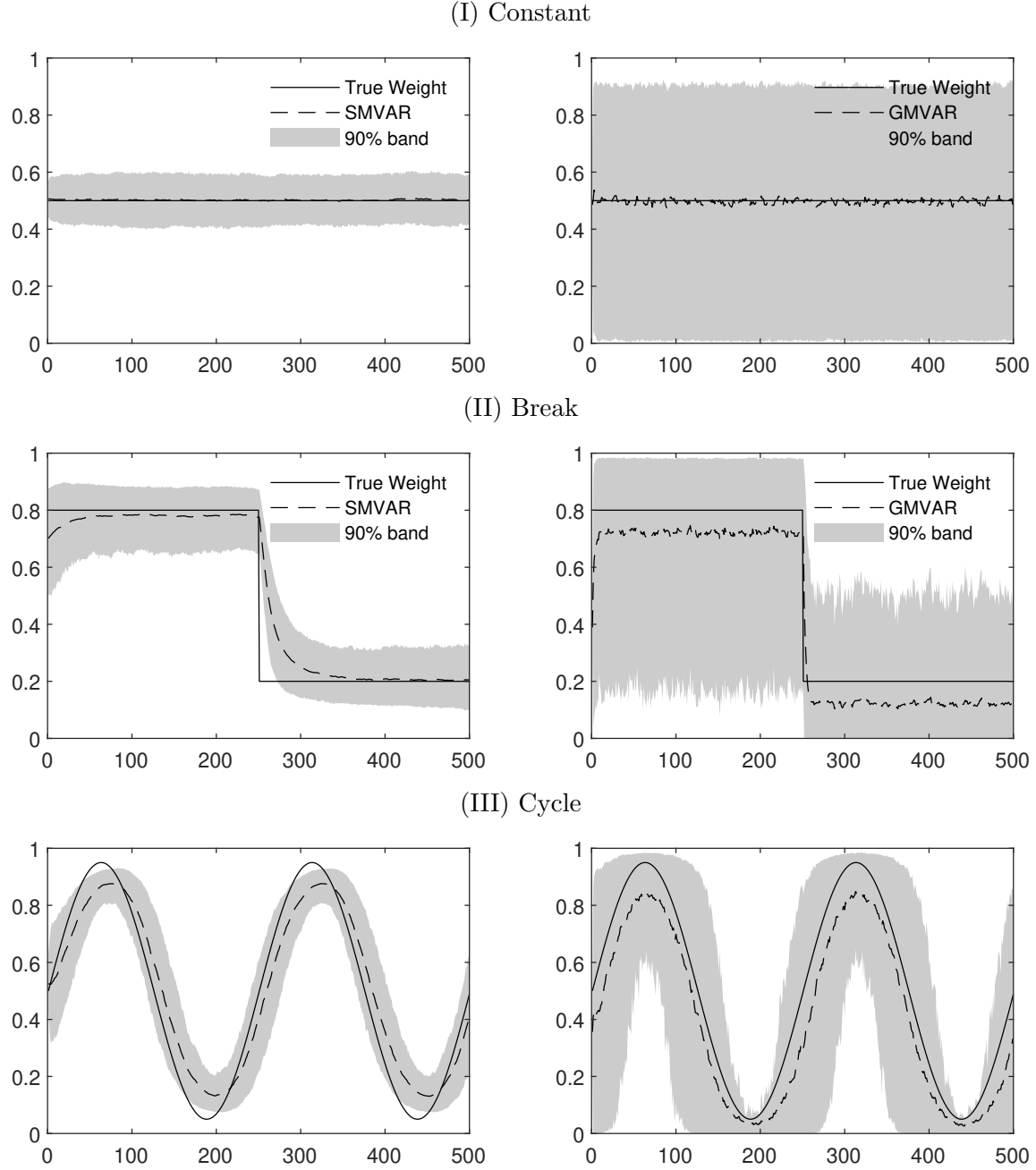
Figure 1: Filtered Mixture Weights
