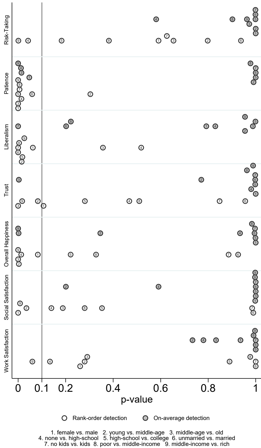
FIGURE 6: Detection analysis in the binary survey.
