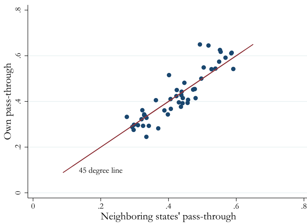
Figure B3: Relationship between states' own pass-through and average pass-through in adjacent states
