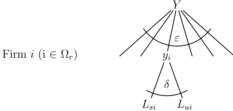
Figure 2: Structure of the Aggregate Production Function
