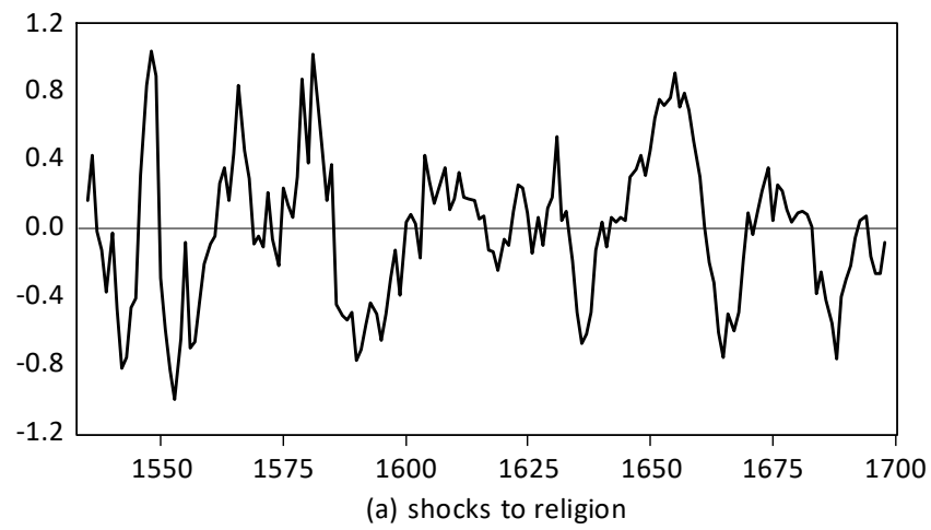
Figure 4: Structural shocks
