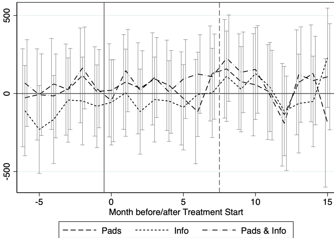
Figure A.1: Earnings over Time
