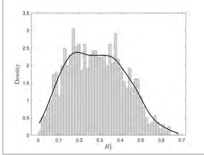
Figure DS5: Histogram and density function of the R-squared of the panel regression over 2002m1-2021m12 ( T = 240 ) and n = 1775
