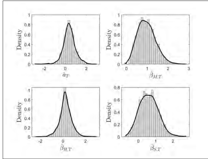
Figure DS4: Histogram and density function of the coefficients of the panel regression over 2002m1-2021m12 ( T = 240 ) and n = 1775
