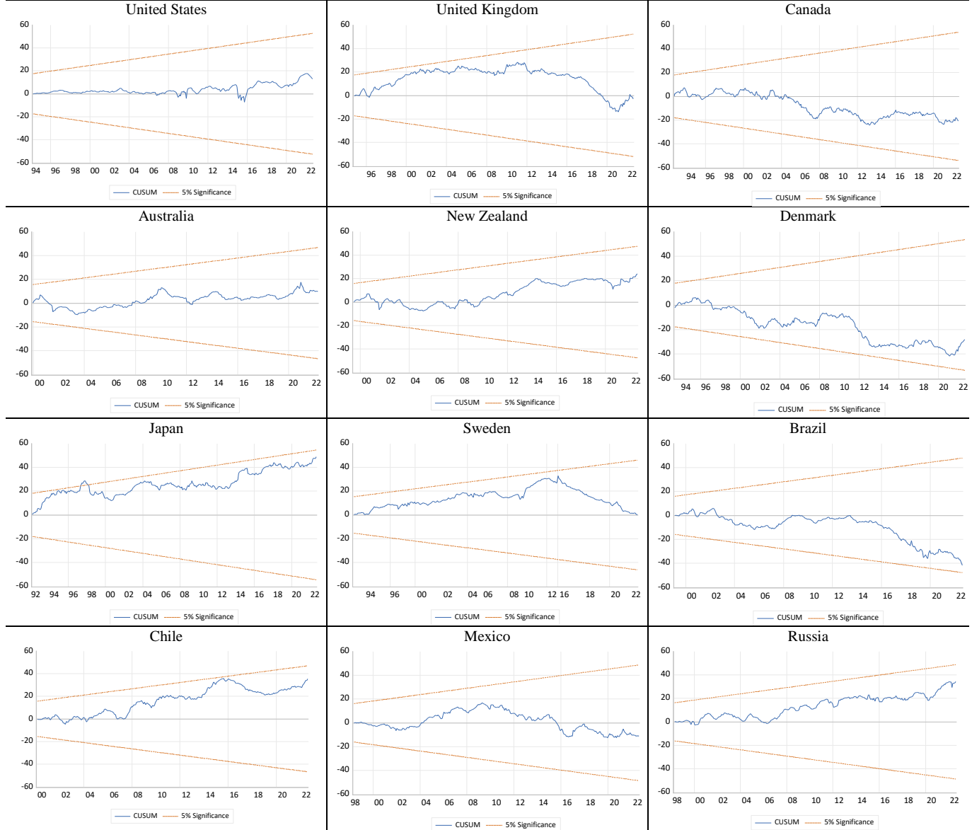
Figure B1. CUSUM Graphs
