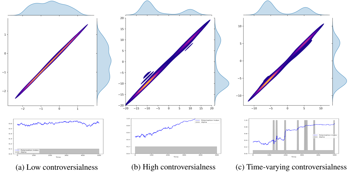
Figure 3: Simulated distribution of stances
