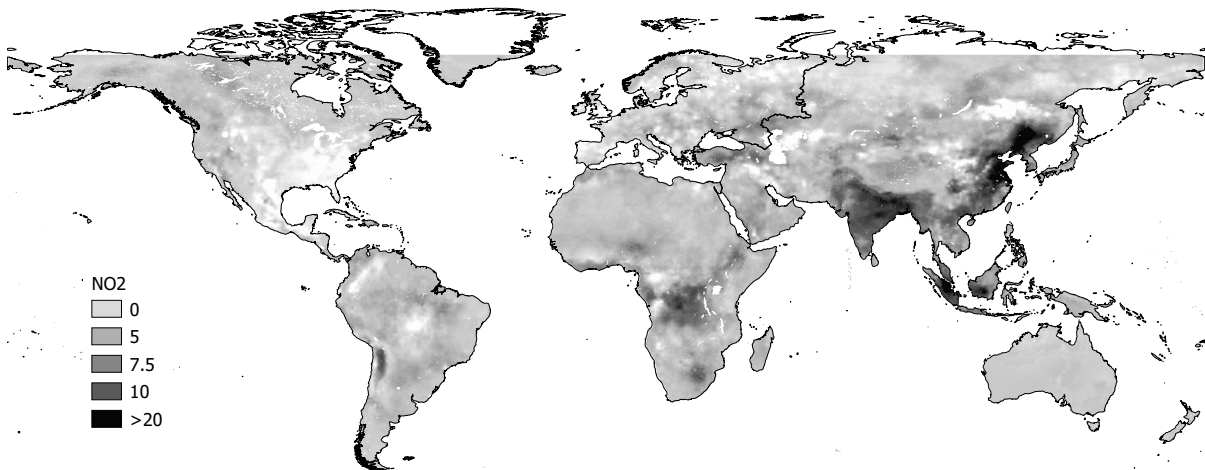
(a) NO 2 concentration in 2010
