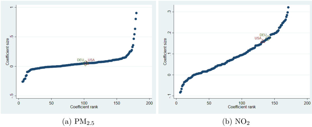
Figure 7: Distribution of country-specific density coefficients
