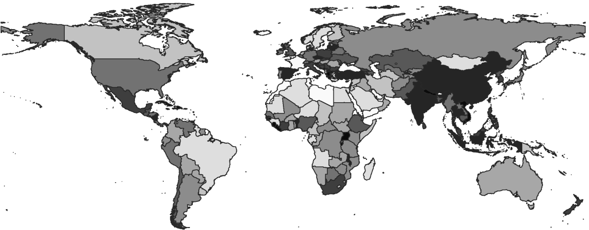
Figure 6: Density coefficients for PM_{2.5} by country
