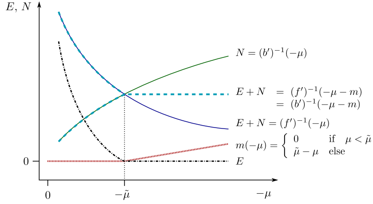
FIGURE 2. The social cost of carbon determine whether the non-negativity constraint on emissions binds. As long as \text{SCC-E} < -\tilde{\mu} , we have E > 0 .
