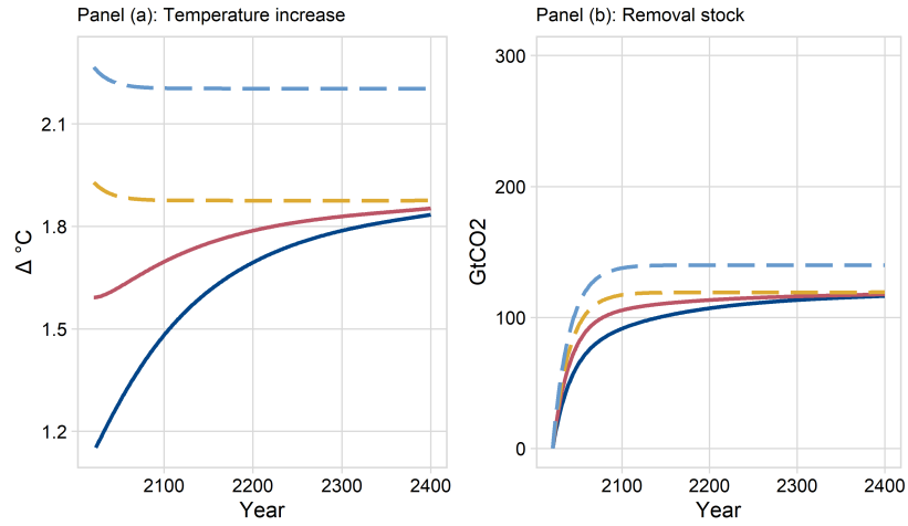
FIGURE A.7. Alternative calibration ( \delta = 5\% , r = 1.5\% , \tilde{\beta} = 0.035 ): Temperature increase and removal stocks in scenarios with and without overshooting.
