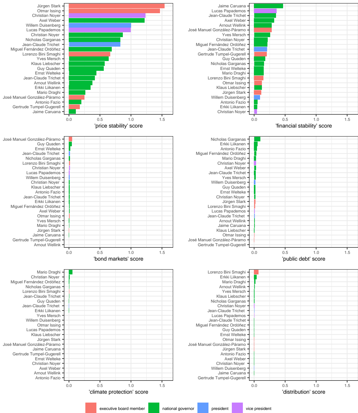
Figure 10: Individual level 1999-2008
