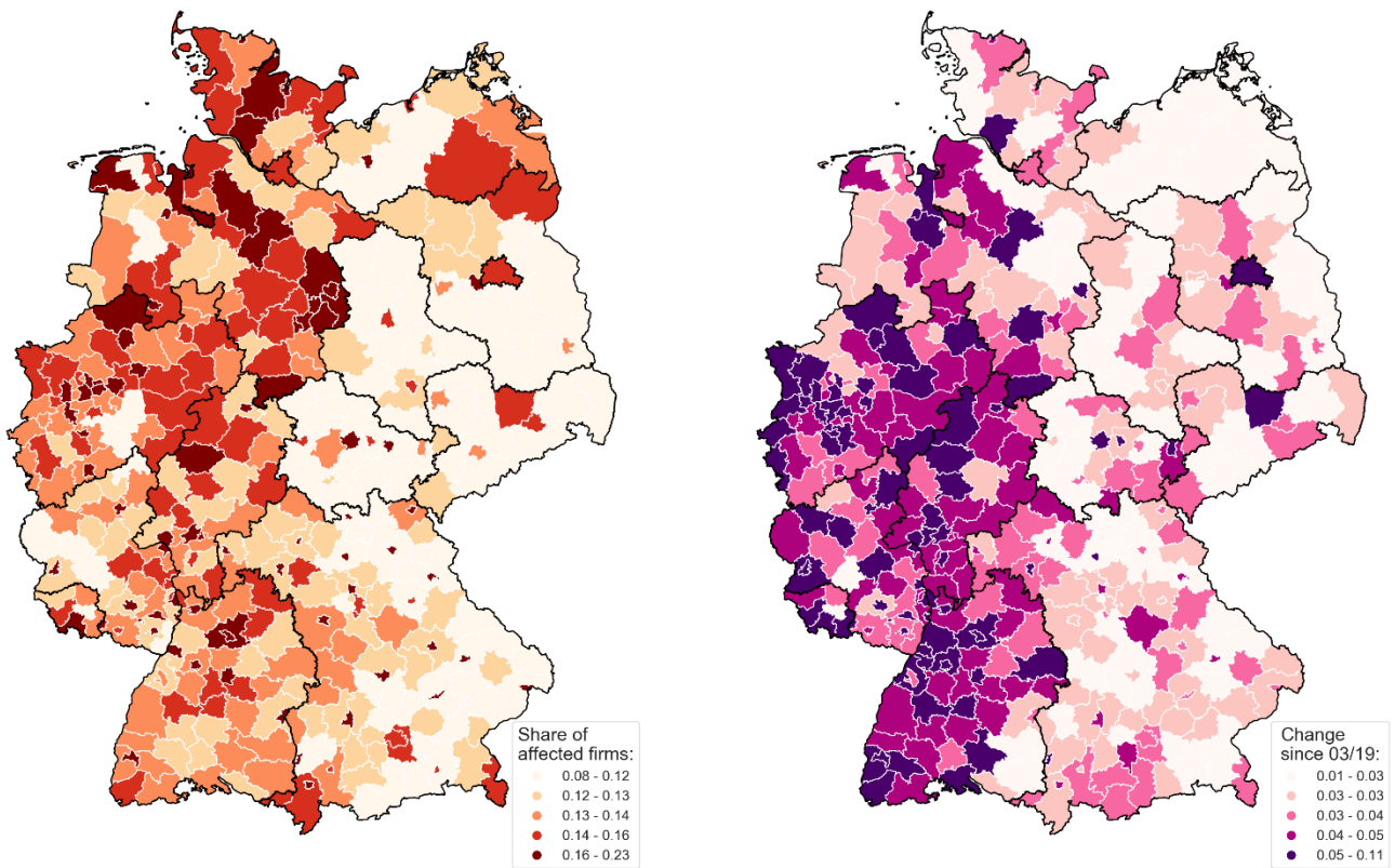
Figure 5: Share (left) and change (right) of companies with at least one "coronavirus" web reference by districts.
