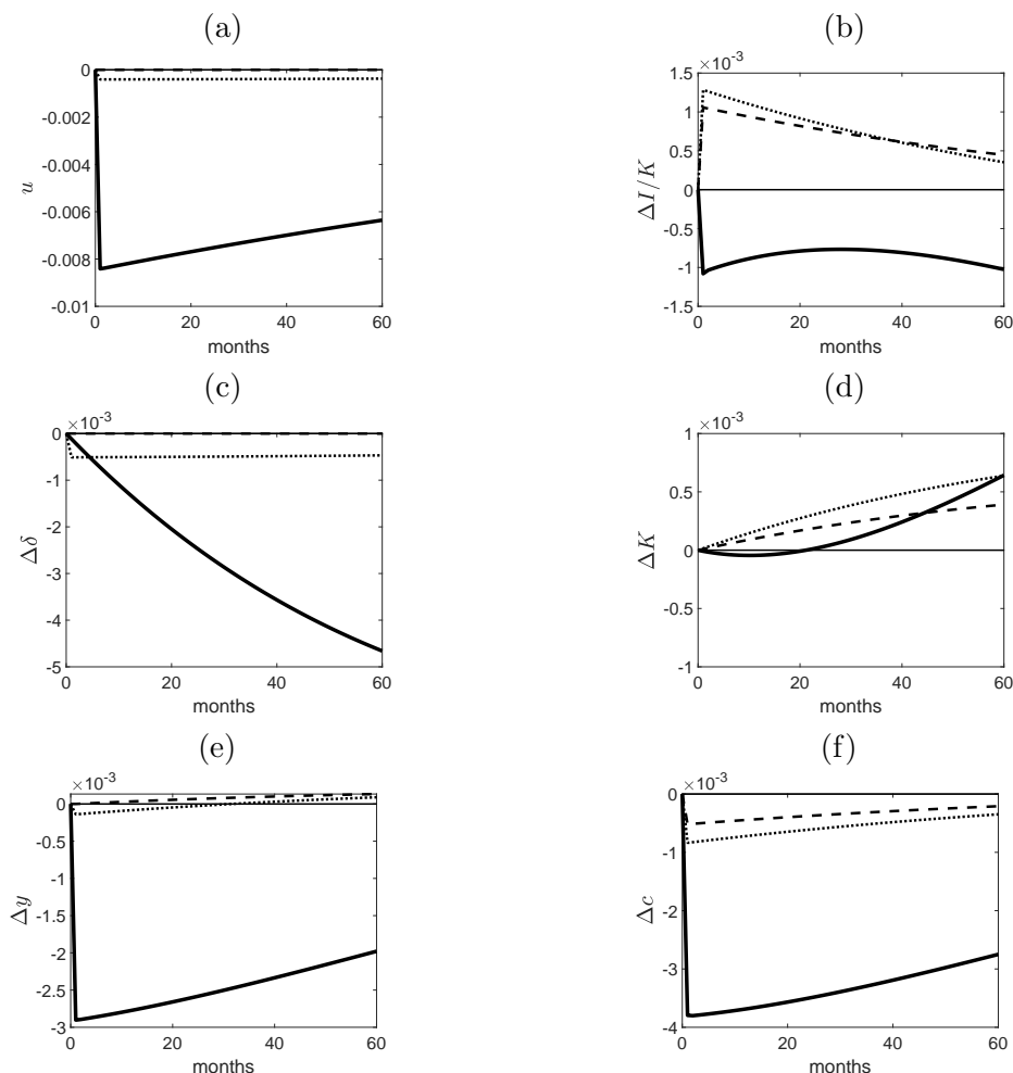
Figure 5: Model-implied IR to uncertainty shocks: macro growth
