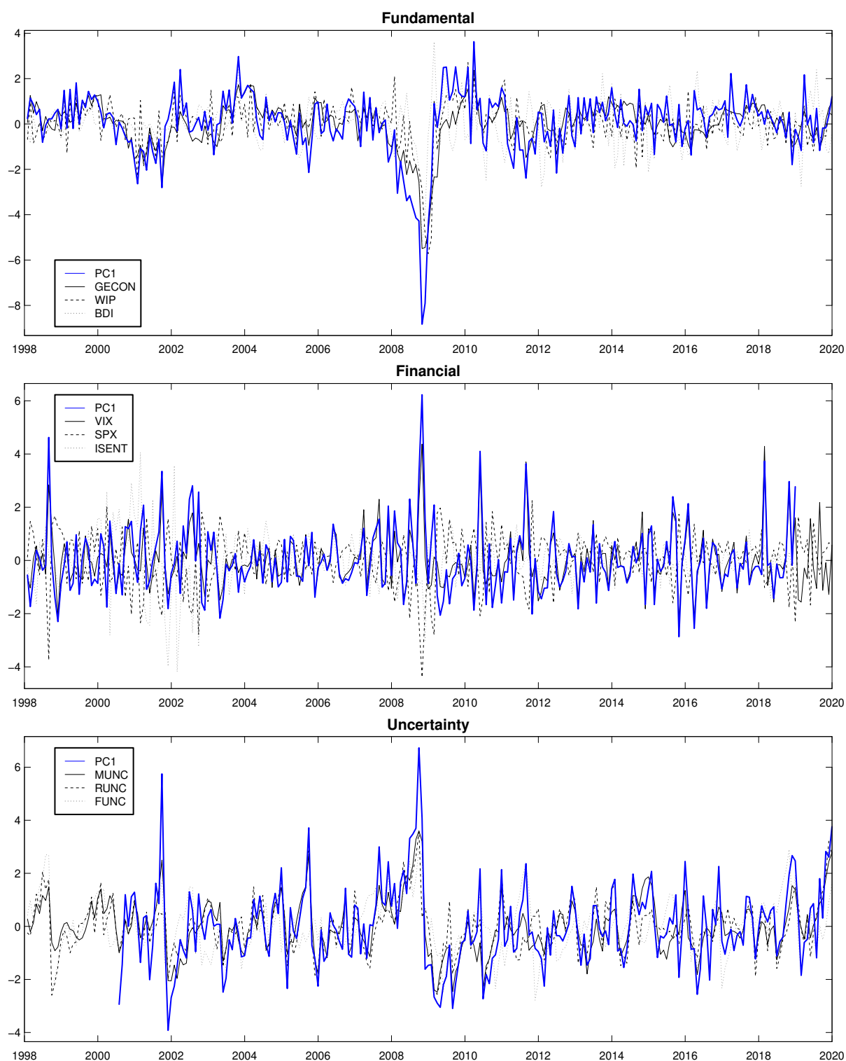
Figure C.6: First PCs of LF fundamental, financial, and uncertainty driver variables and standardized variables of the respective set of drivers that exhibit the highest correlation to the first PC. Note that for our Granger causality analysis, we exclude variables for which data is not available over the full (sub-)sample period prior to running the PC analysis, such that the respective PC always covers the full (sub-)sample period.
