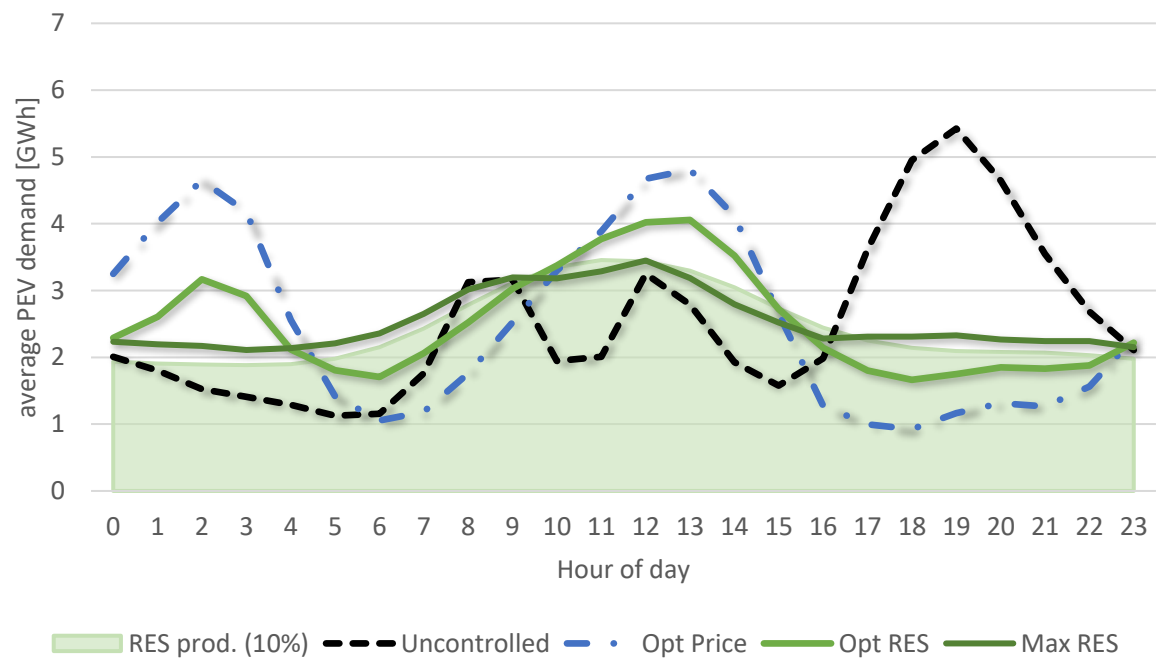
Figure 2: Average PEV-demand (lines) and RES provision (area) for a) Germany and b) France in 2030
