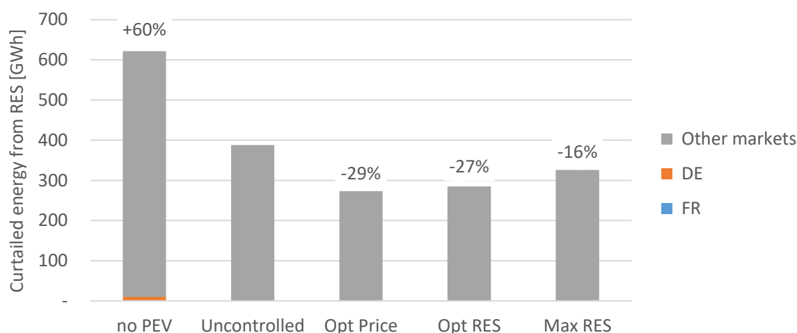
Figure 7: Cumulative curtailment of RES across all simulated markets under the different scenarios in 2030. Percentages relative to Uncontrolled.
