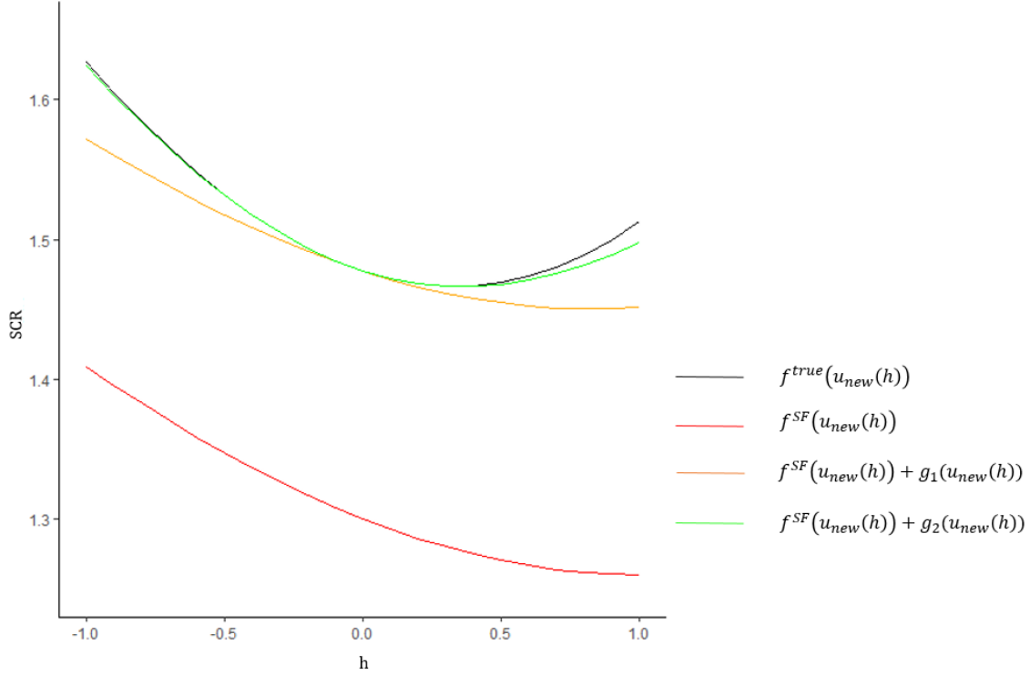
Figure 2: SCRs on the basis of the different risk measurement functions evaluating u_{\text{new}}(h) as in Eq. (18).
