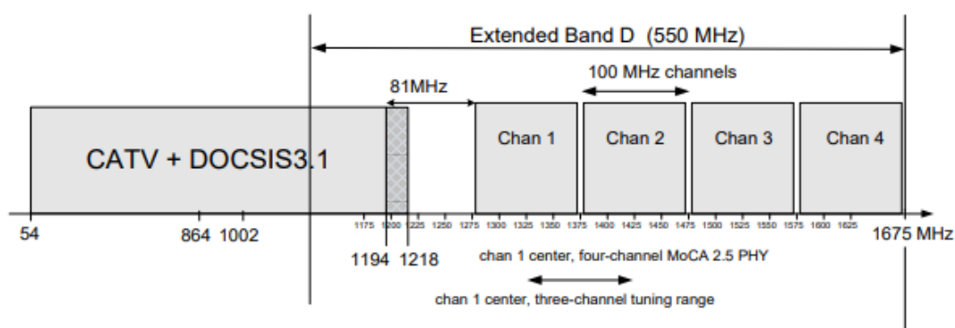
Figure 4-7: MoCA 2.5 extended band D frequency plan
