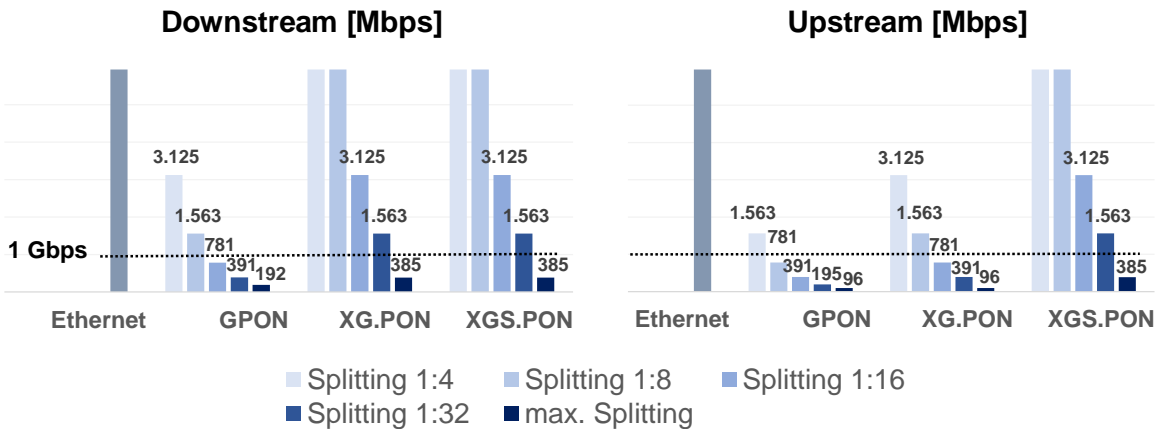
Figure 4-10: Ethernet over Fibre and x.PON series – Individual transmission speeds for end users in different splitting ratios (at busy hour = 20% simultaneity) 75
