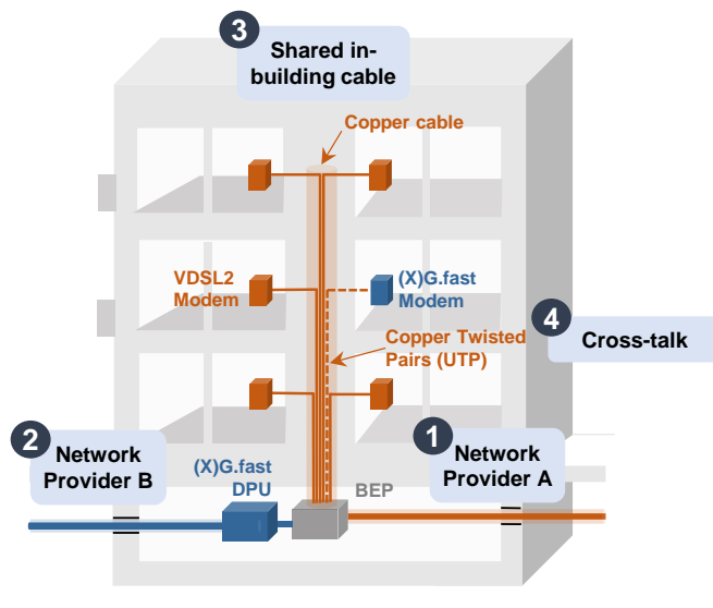
Figure 4-4: Technical issues of upgrading (from FTTC to FTTB) a single apartment in a multi-dwelling unit using the same in-building copper cables
