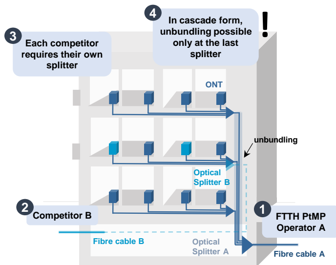
Figure 4-11: Challenges of sharing and unbundling in Point-to-Multipoint (PtMP) network architectures with passive optical splitters in a cascade form
