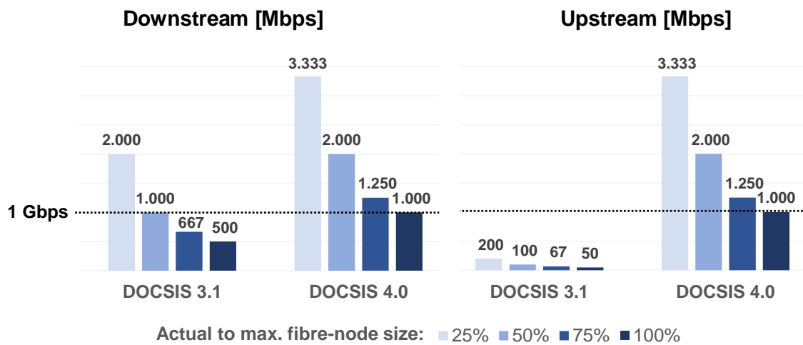
Figure 4-5: DOCSIS 3.1 and DOCSIS 4.0 – Individual transmission speeds for end users for different fibre-node sizes (at busy hour = 20% simultaneity) 48
