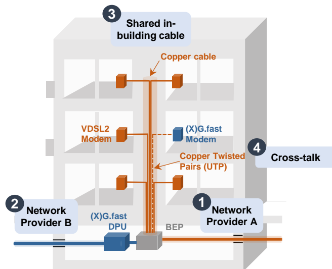
Figure 4-4: Technical issues of upgrading (from FTTC to FTTB) a single apartment in a multi-dwelling unit using the same in-building copper cables
