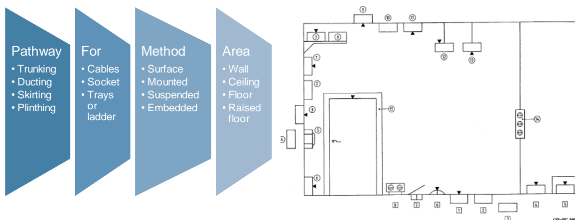
Figure 4-14: Overview of cable trunking and ducting systems
