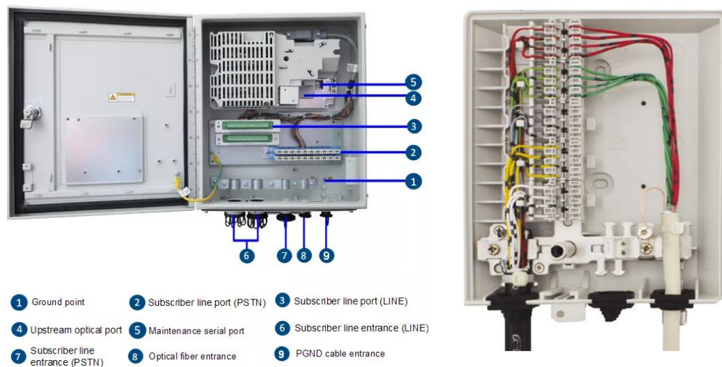
Figure 4-1: G.fast distribution point unit (DPU) and building entry unit (BEP)
