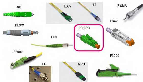
Figure 4-15: Fibre cable connectors
