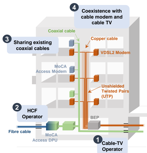
Figure 4-8: Multimedia over Coax Alliance (MoCA) access
