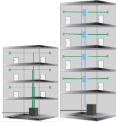
Figure 4-2: Typical in-building cabling structures for multi-dwelling buildings
