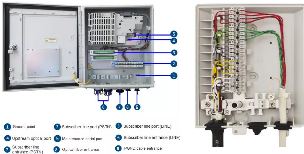
Figure 4-1: G.fast distribution point unit (DPU) and building entry unit (BEP)
