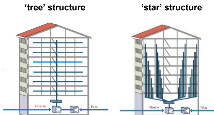
Figure 4-6: Typical in-building cabling structures in multi-dwelling units in Germany
