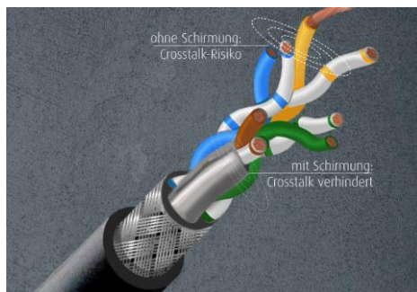
Figure 4-3: Copper twisted pairs with and without shielding and 'cross-talk'
