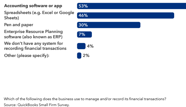
FIGURE 7: SOFTWARE USAGE
