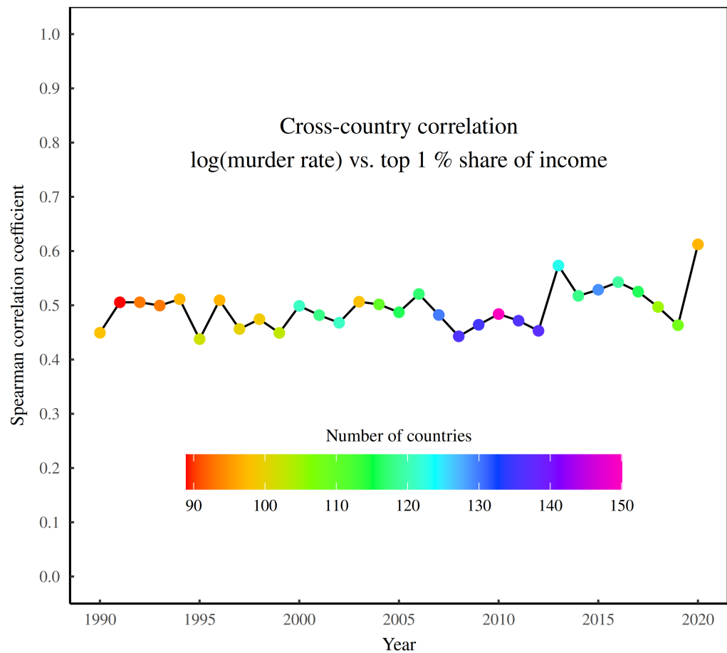
Figure 5: Not a fluke correlation
