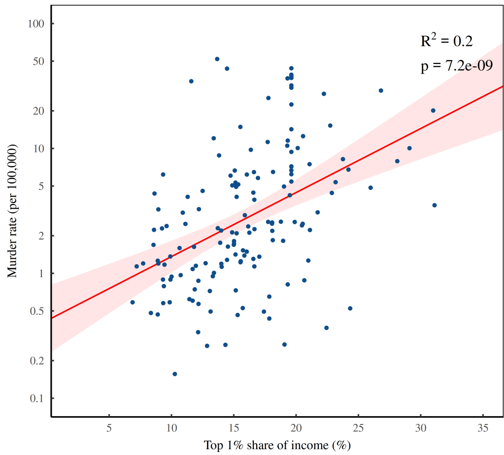
Figure 1: The murder rate vs. the top 1% share of income across countries Sources and methods
