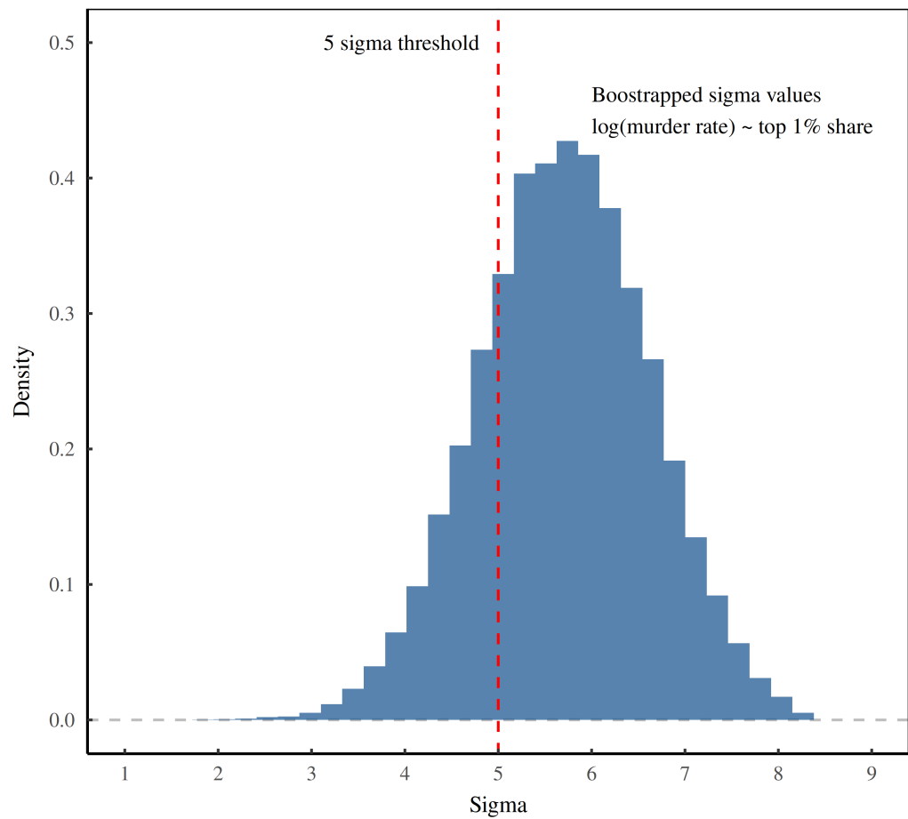
Figure 4: Bootstrapping statistical significance
