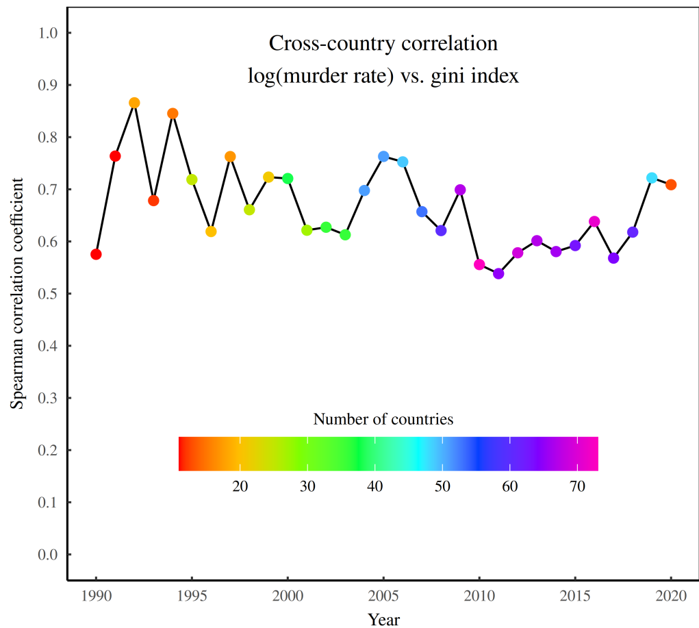
Figure 7: Still not a fluke correlation
