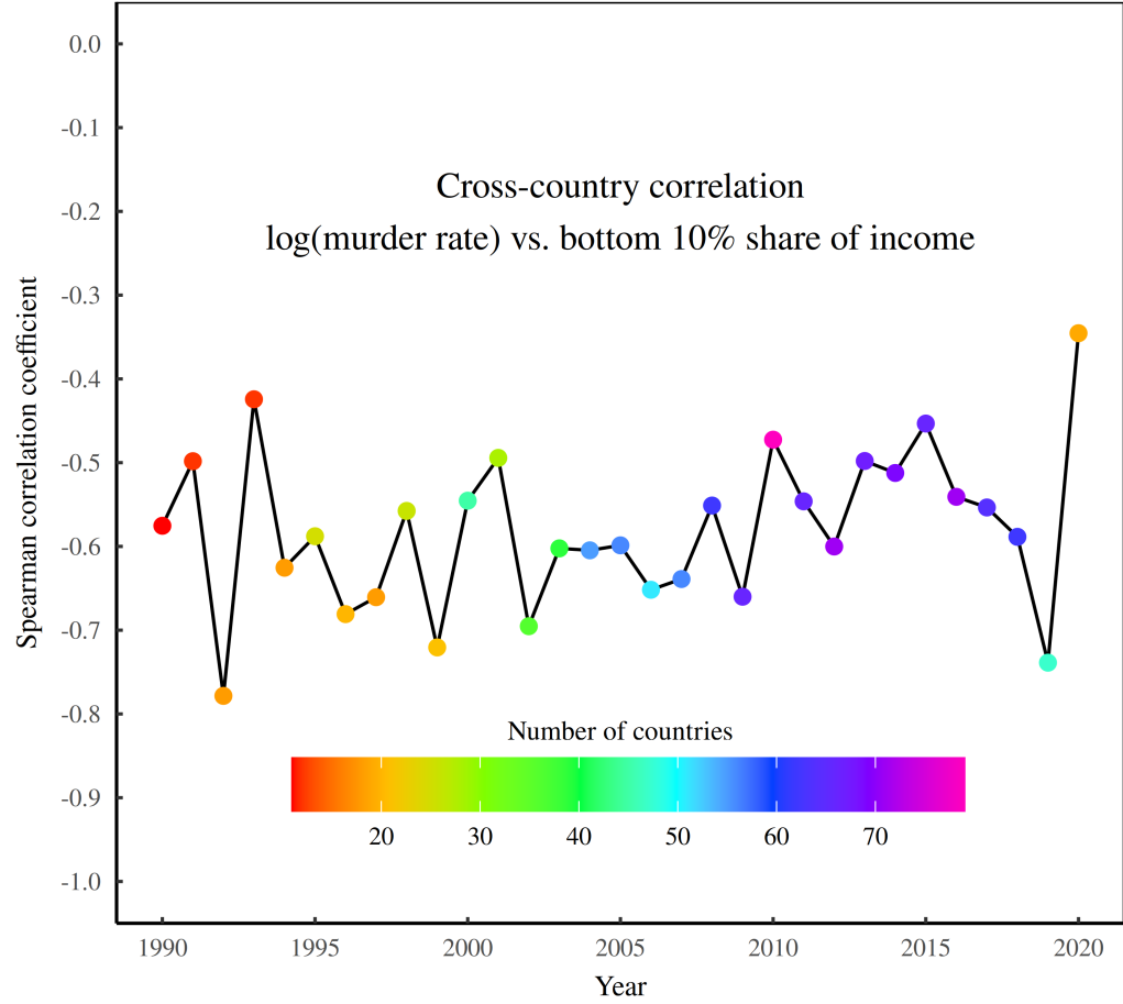
Figure 9: Really still not a fluke correlation
