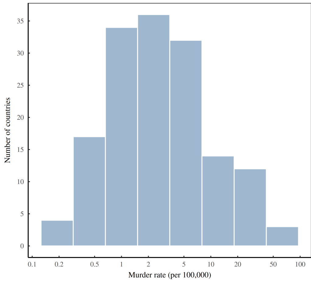
Figure 3: Across countries, murder rates are log-normally distributed
