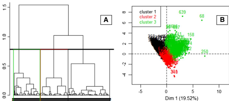
Fig. 3 Cluster dendrogram and clusters graphic representation
